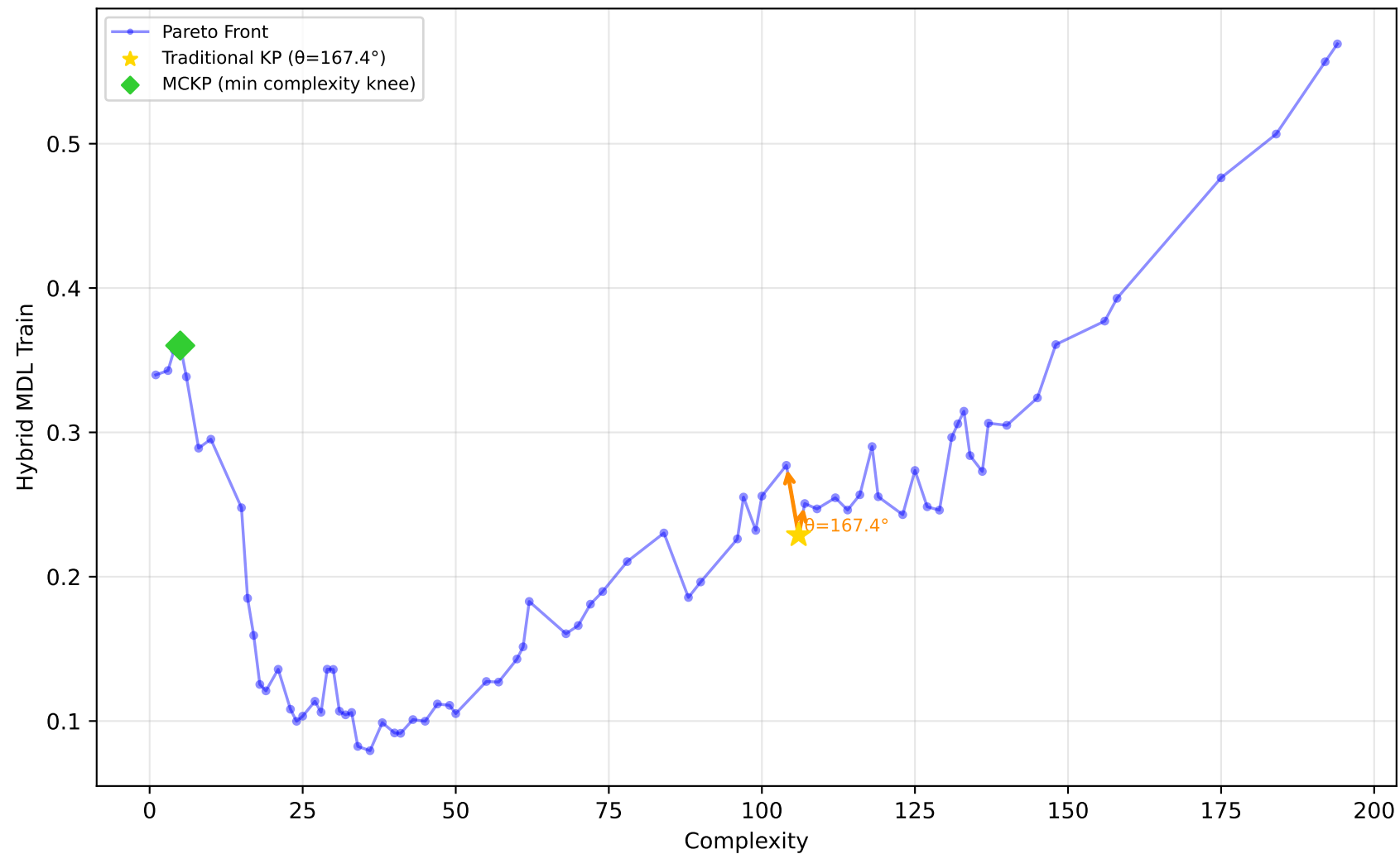
556_analcatdata_apnea2 - Run 15 - MVP - Hybrid MDL Train \lambda_1=0.00, \lambda_2=0.00, \lambda_3=0.00 | Difficulty: 1.00 | Method: hmr
