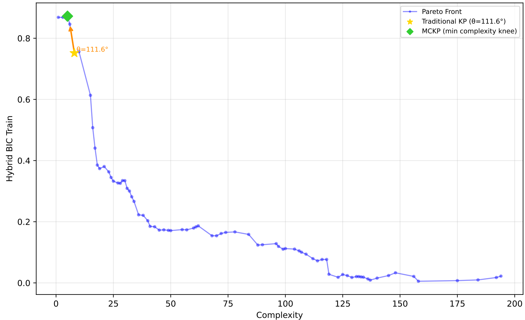
556_analcatdata_apnea2 - Run 15 - SVP - Hybrid BIC Train \lambda_1=0.00, \lambda_2=0.00, \lambda_3=0.00 | Difficulty: 1.00 | Method: hmr
