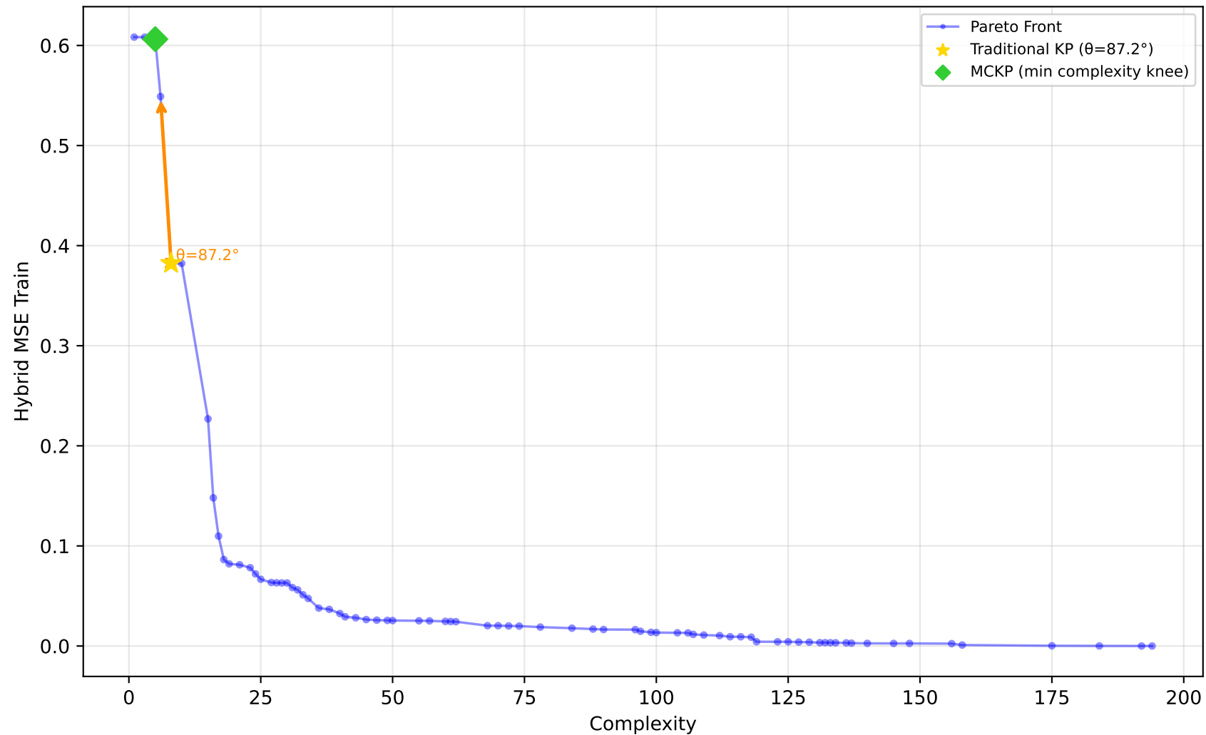
556_analcatdata_apnea2 - Run 15 - SVP - Hybrid MSE Train \lambda_1=0.00, \lambda_2=0.00, \lambda_3=0.00 | Difficulty: 1.00 | Method: hmr
