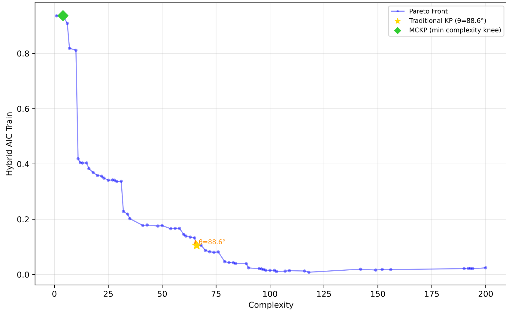
556_analcatdata_apnea2 - Run 16 - MVP - Hybrid AIC Train \lambda_1=0.00, \lambda_2=0.00, \lambda_3=0.00 | Difficulty: 1.00 | Method: hmr
