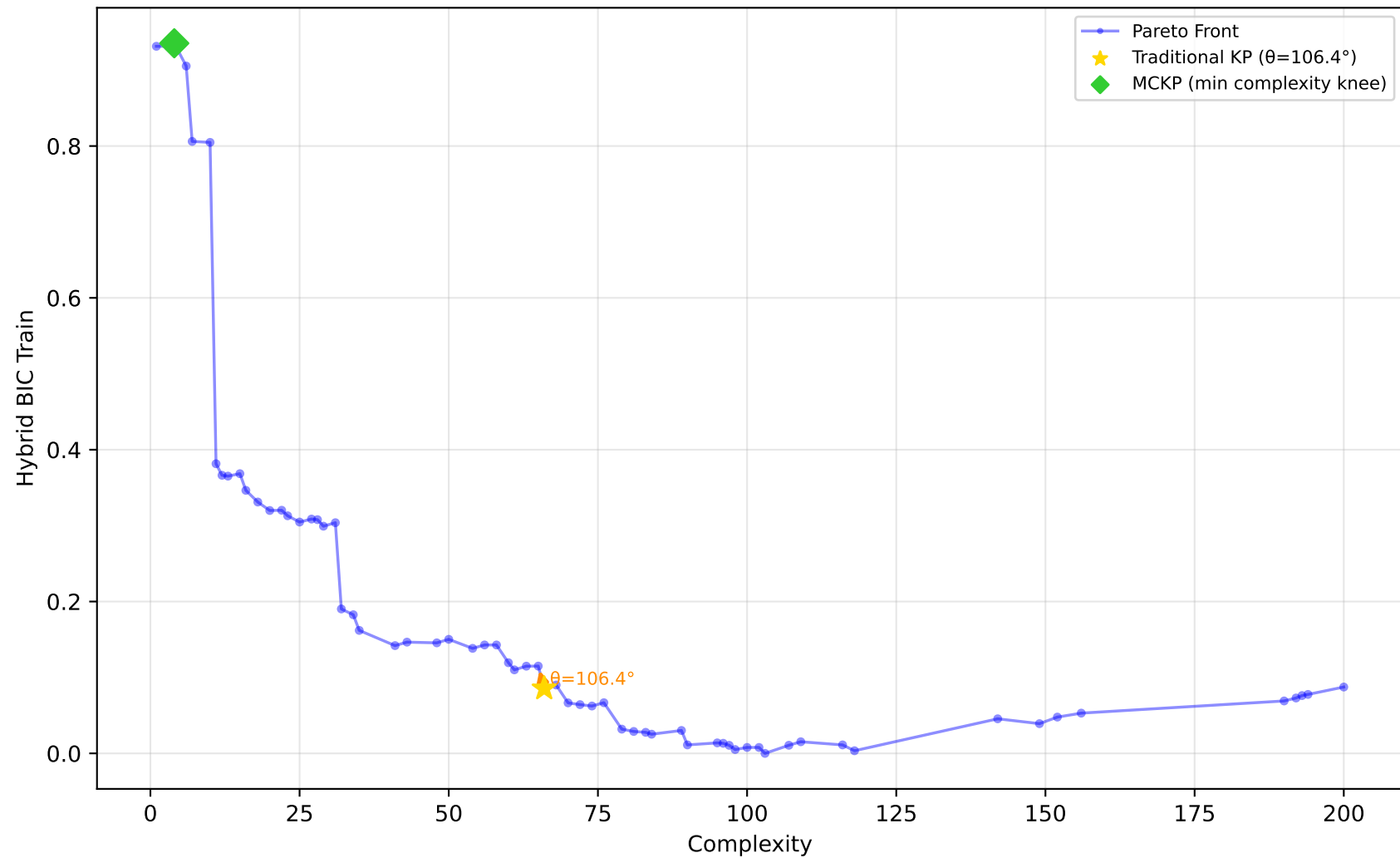
556_analcatdata_apnea2 - Run 16 - MVP - Hybrid BIC Train \lambda_1=0.00, \lambda_2=0.00, \lambda_3=0.00 | Difficulty: 1.00 | Method: hmr
