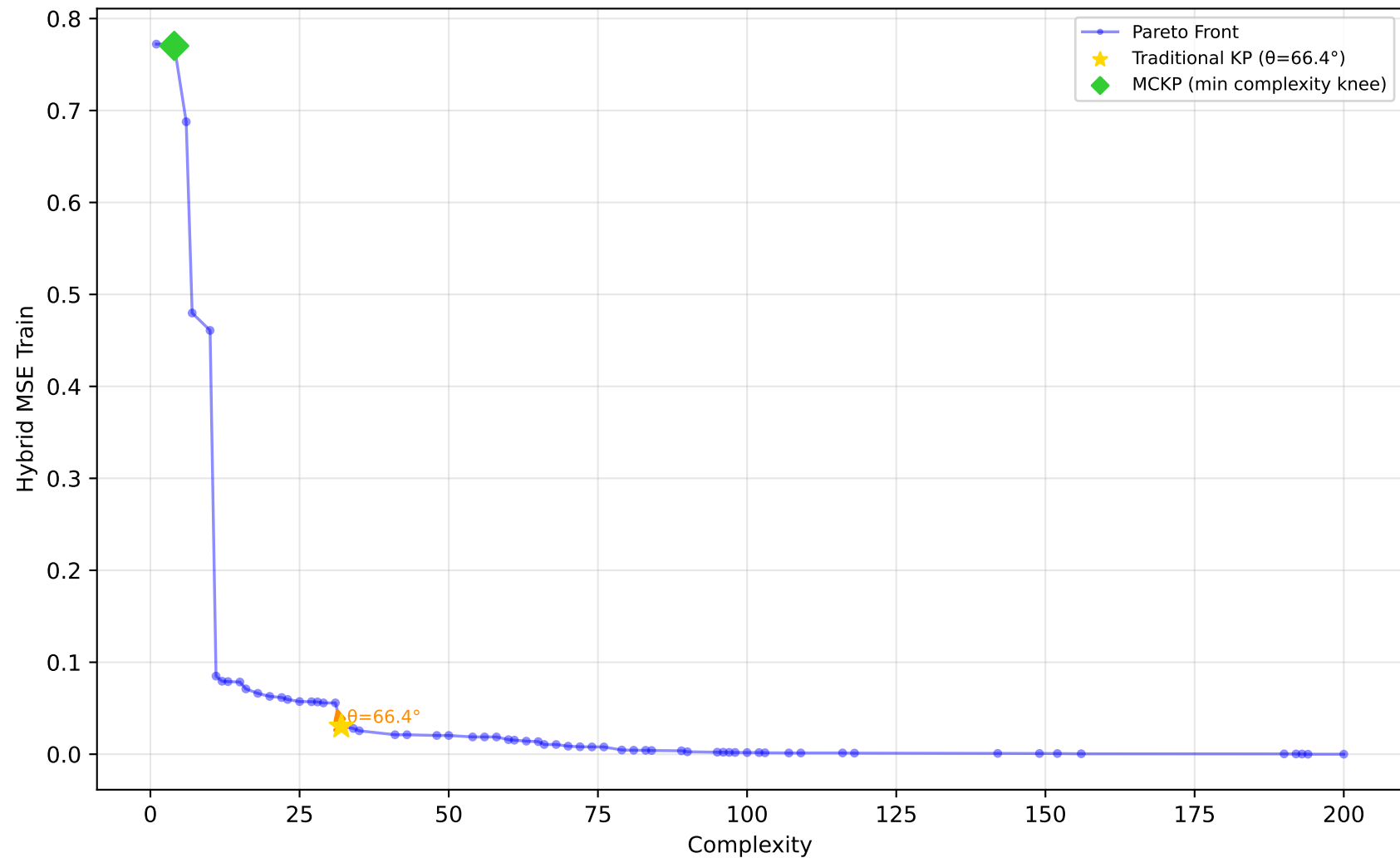
556_analcatdata_apnea2 - Run 16 - MVP - Hybrid MSE Train \lambda_1=0.00, \lambda_2=0.00, \lambda_3=0.00 | Difficulty: 1.00 | Method: hmr
