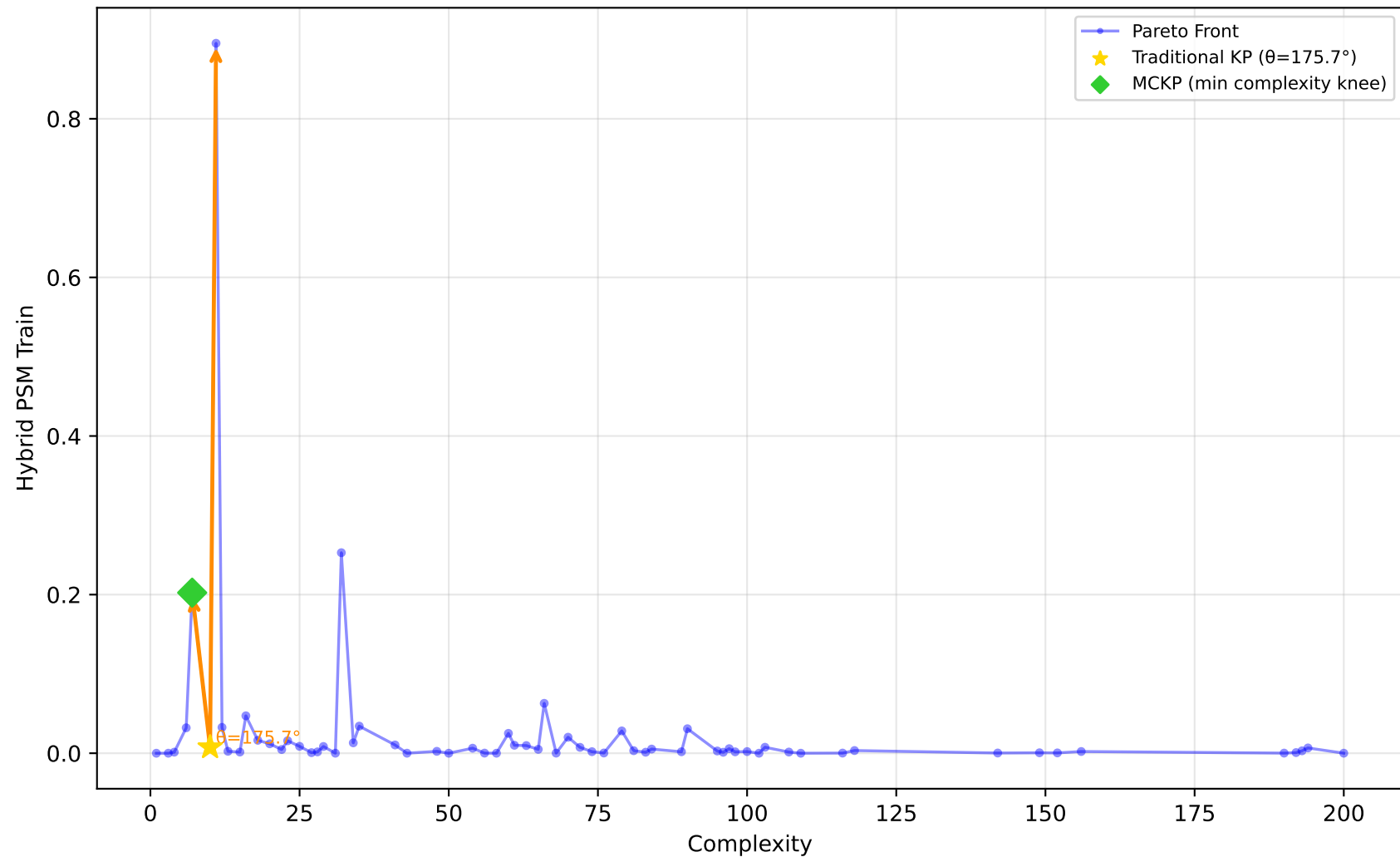
556_analcatdata_apnea2 - Run 16 - MVP - Hybrid PSM Train \lambda_1=0.00, \lambda_2=0.00, \lambda_3=0.00 | Difficulty: 1.00 | Method: hmr
