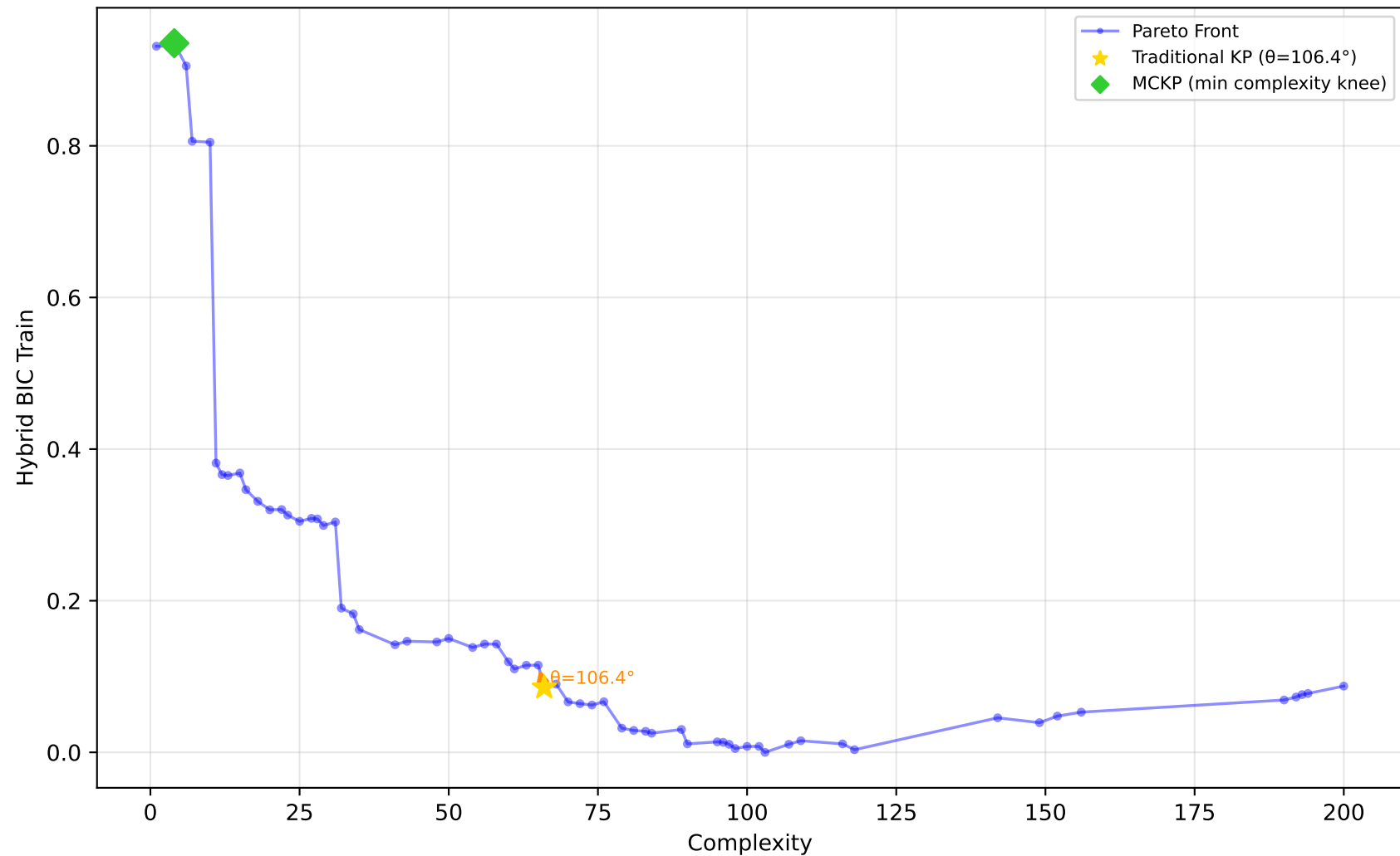
556_analcatdata_apnea2 - Run 16 - SVP - Hybrid BIC Train \lambda_1=0.00, \lambda_2=0.00, \lambda_3=0.00 | Difficulty: 1.00 | Method: hmr
