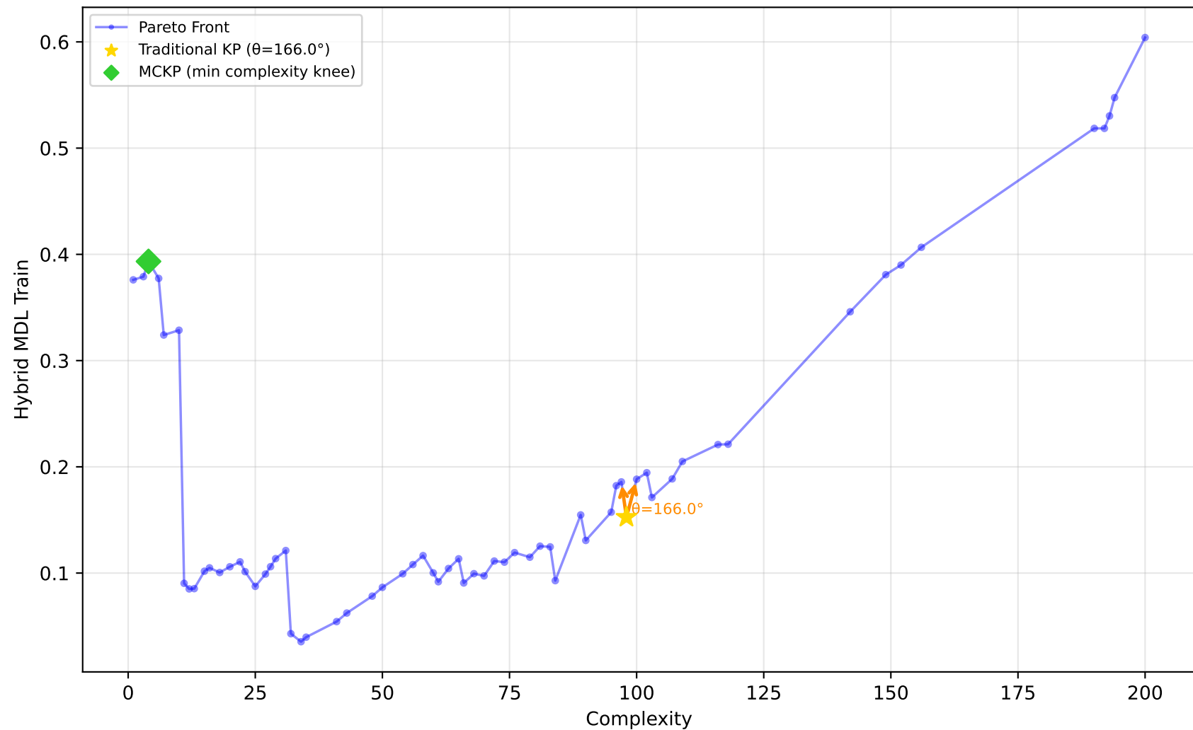
556_analcatdata_apnea2 - Run 16 - SVP - Hybrid MDL Train \lambda_1=0.00, \lambda_2=0.00, \lambda_3=0.00 | Difficulty: 1.00 | Method: hmr
