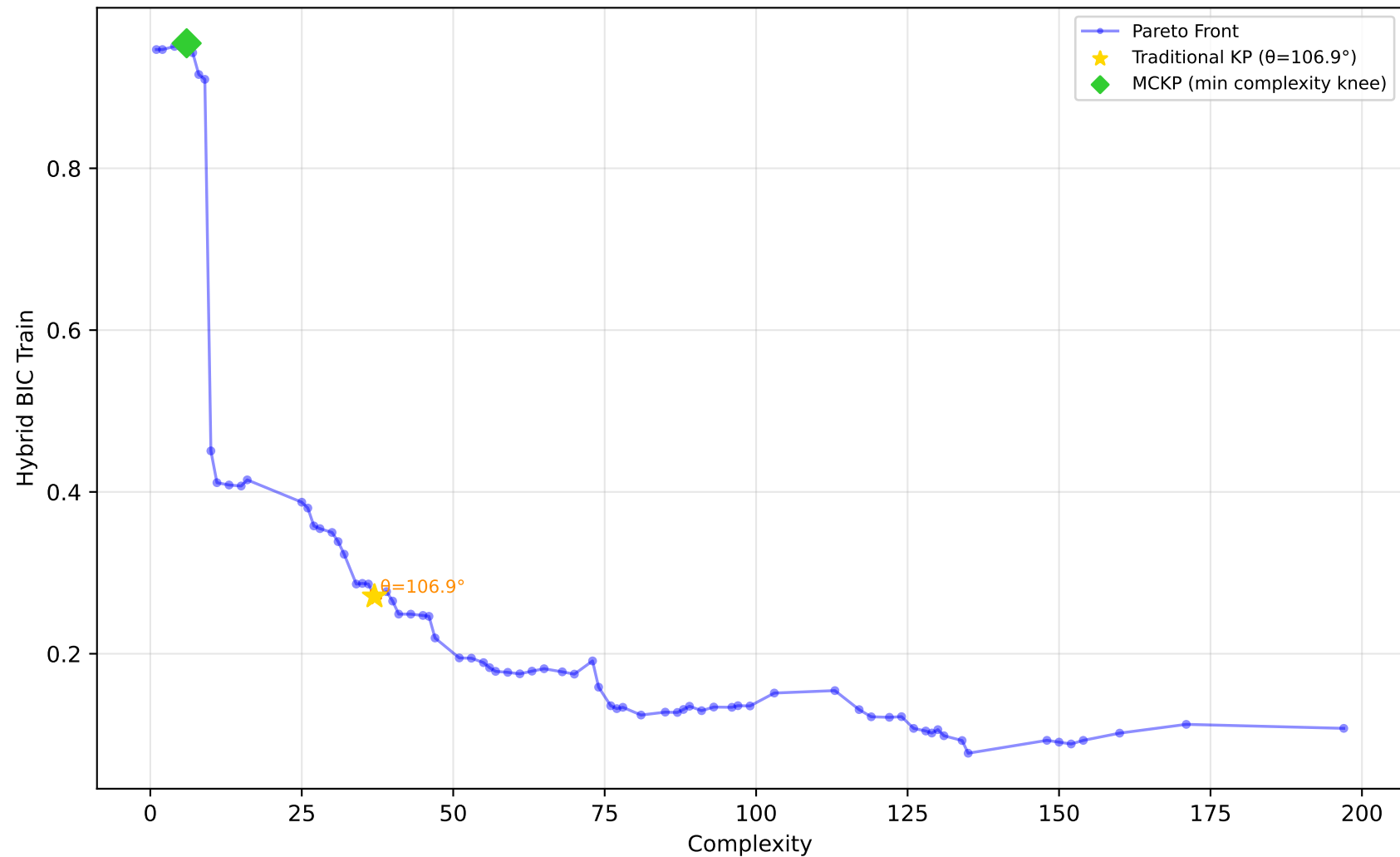
556_analcatdata_apnea2 - Run 17 - MVP - Hybrid BIC Train \lambda_1=0.00, \lambda_2=0.00, \lambda_3=0.00 | Difficulty: 0.86 | Method: hmr
