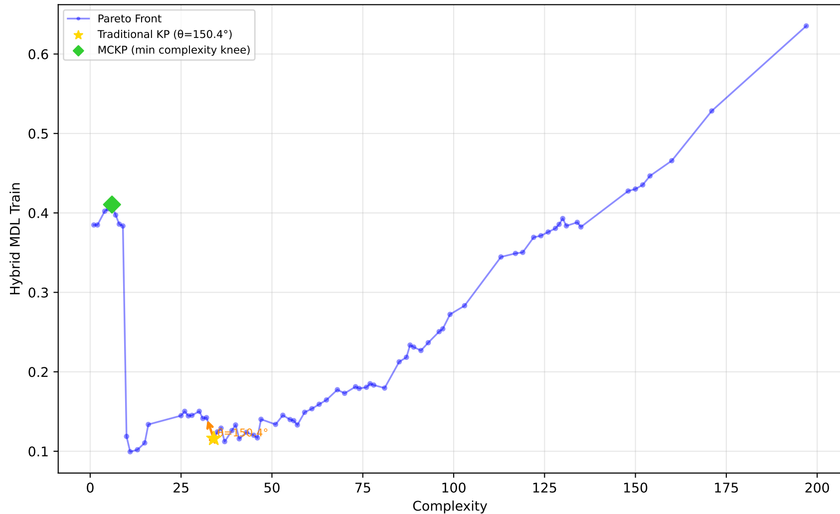
556_alanctdata_apnea2 - Run 17 - SVP - Hybrid MDL Train \lambda_1=0.00, \lambda_2=0.00, \lambda_3=0.00 | Difficulty: 0.86 | Method: hmr
