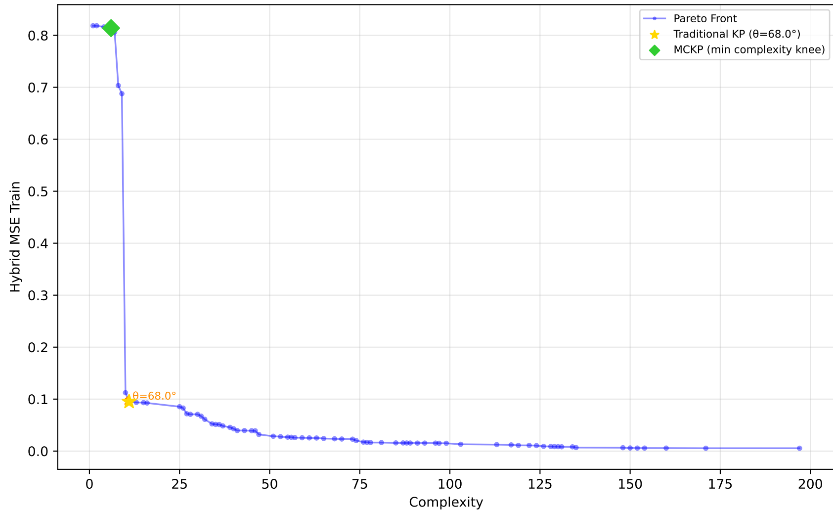
556_analcatdata_apnea2 - Run 17 - SVP - Hybrid MSE Train \lambda_1=0.00, \lambda_2=0.00, \lambda_3=0.00 | Difficulty: 0.86 | Method: hmr
