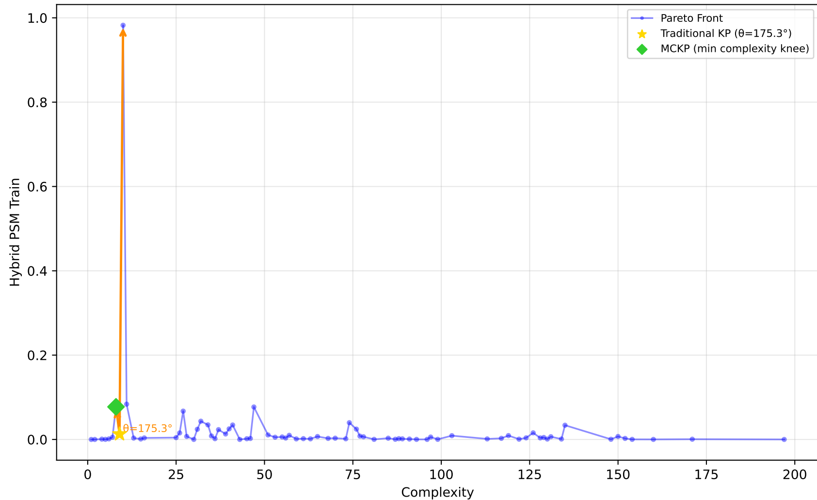
556_analcatdata_apnea2 - Run 17 - SVP - Hybrid PSM Train \lambda_1=0.00 , \lambda_2=0.00 , \lambda_3=0.00 | Difficulty: 0.86 | Method: hmr
