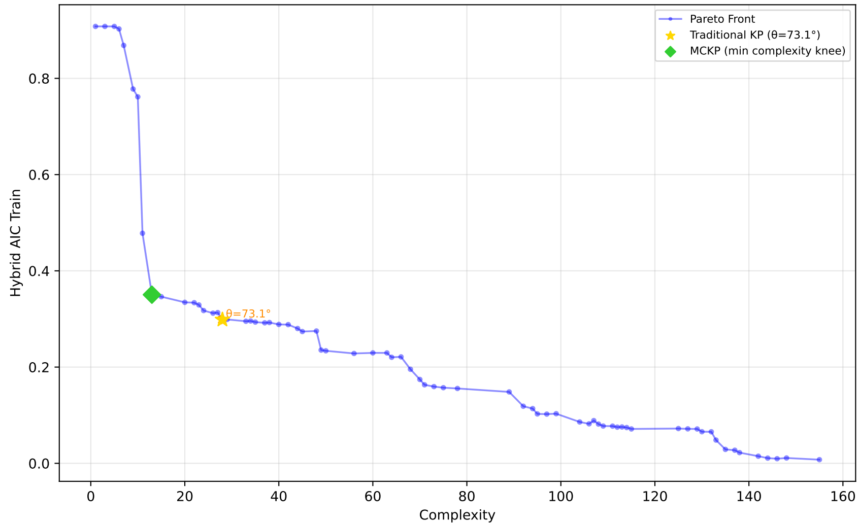
556_analcatdata_apnea2 - Run 18 - MVP - Hybrid AIC Train \lambda_1=0.00, \lambda_2=0.00, \lambda_3=0.00 | Difficulty: 0.86 | Method: hmr
