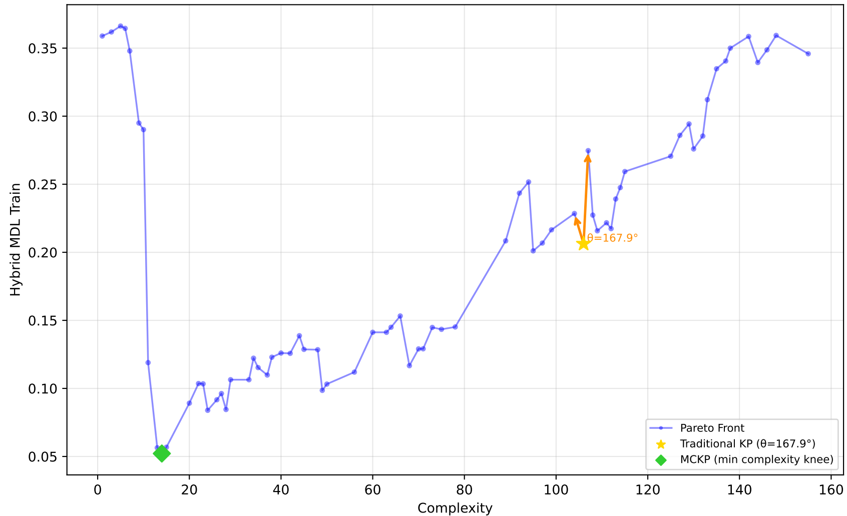
556_analcatdata_apnea2 - Run 18 - MVP - Hybrid MDL Train \lambda_1=0.00 , \lambda_2=0.00 , \lambda_3=0.00 | Difficulty: 0.86 | Method: hmr
