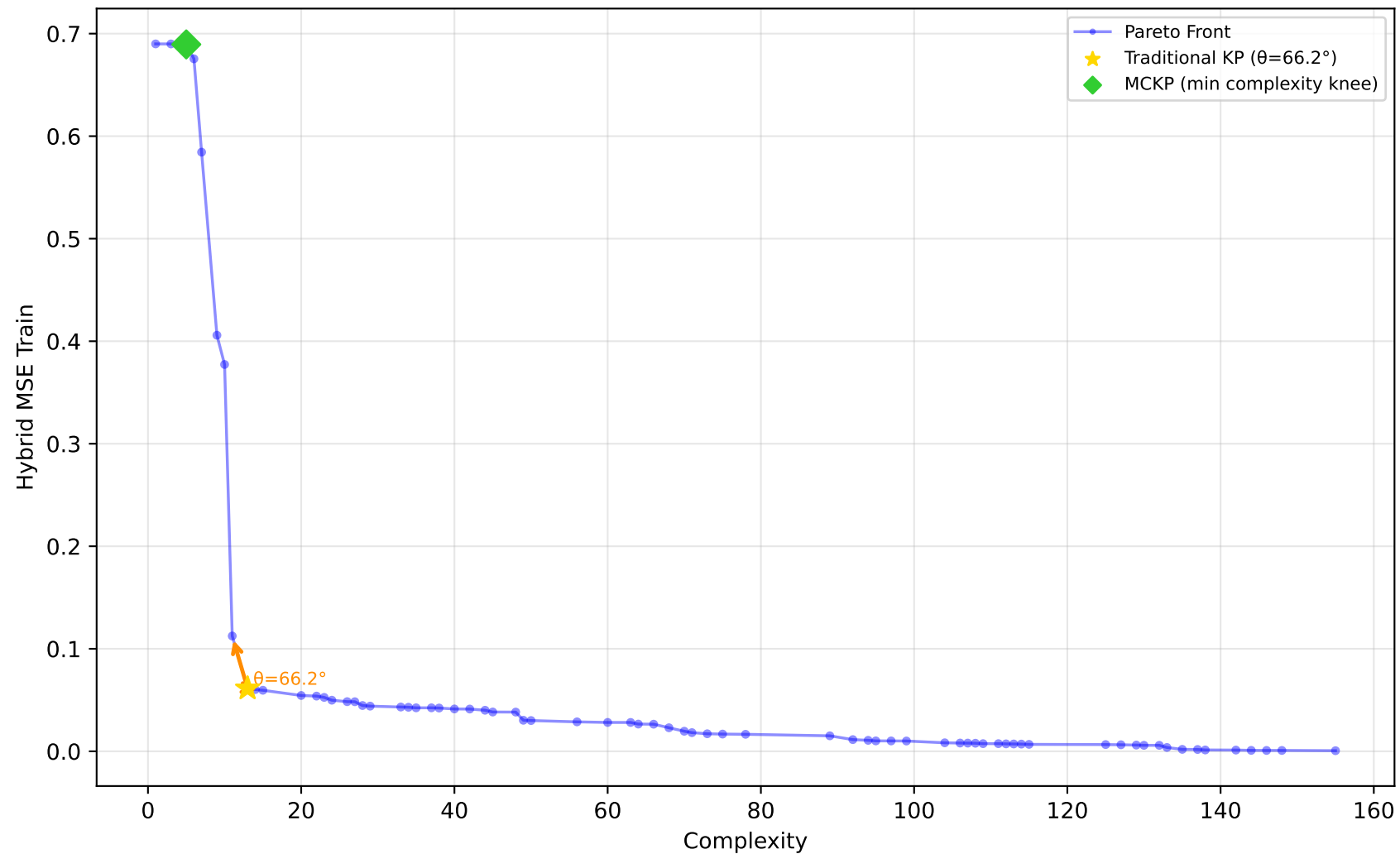
556_analcatdata_apnea2 - Run 18 - MVP - Hybrid MSE Train \lambda_1=0.00, \lambda_2=0.00, \lambda_3=0.00 | Difficulty: 0.86 | Method: hmr
