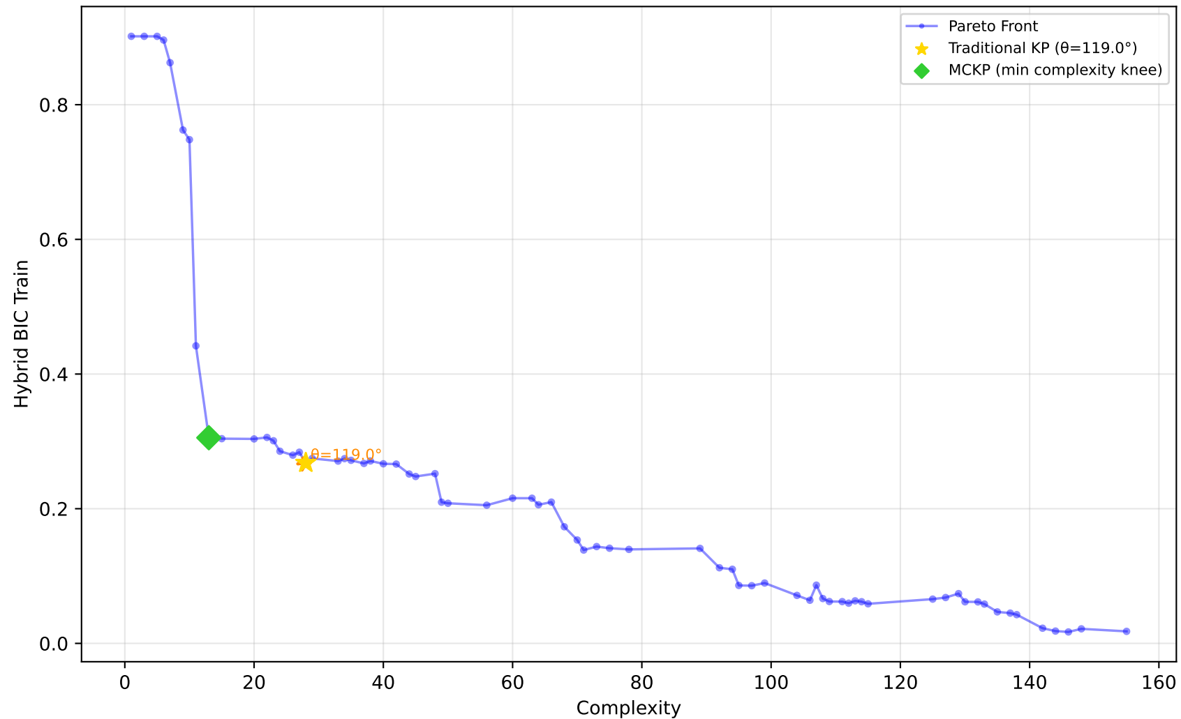
556_analcatdata_apnea2 - Run 18 - SVP - Hybrid BIC Train \lambda_1=0.00, \lambda_2=0.00, \lambda_3=0.00 | Difficulty: 0.86 | Method: hmr
