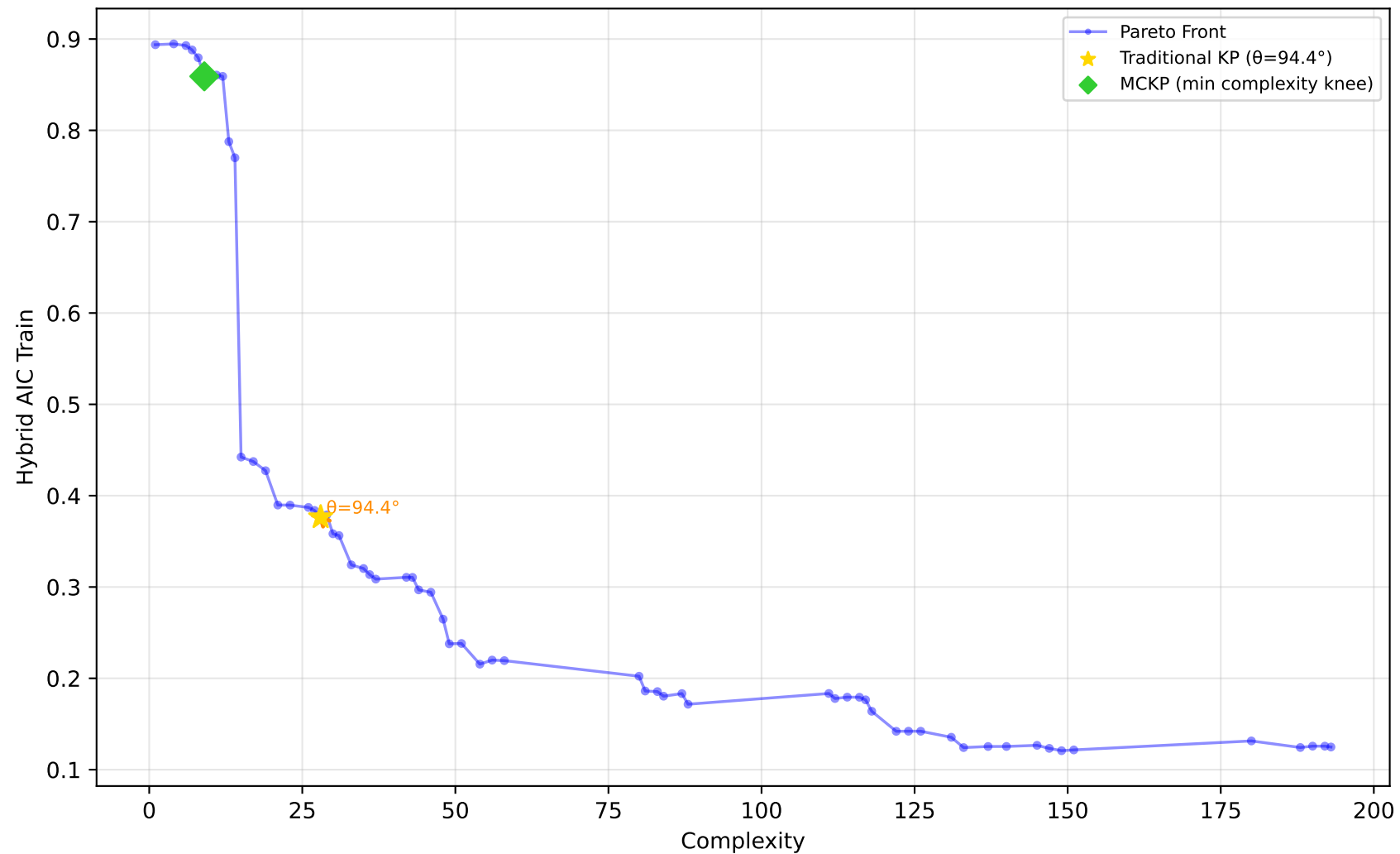
556_analcatdata_apnea2 - Run 19 - MVP - Hybrid AIC Train \lambda_1=0.00, \lambda_2=0.00, \lambda_3=0.00 | Difficulty: 1.00 | Method: hmr
