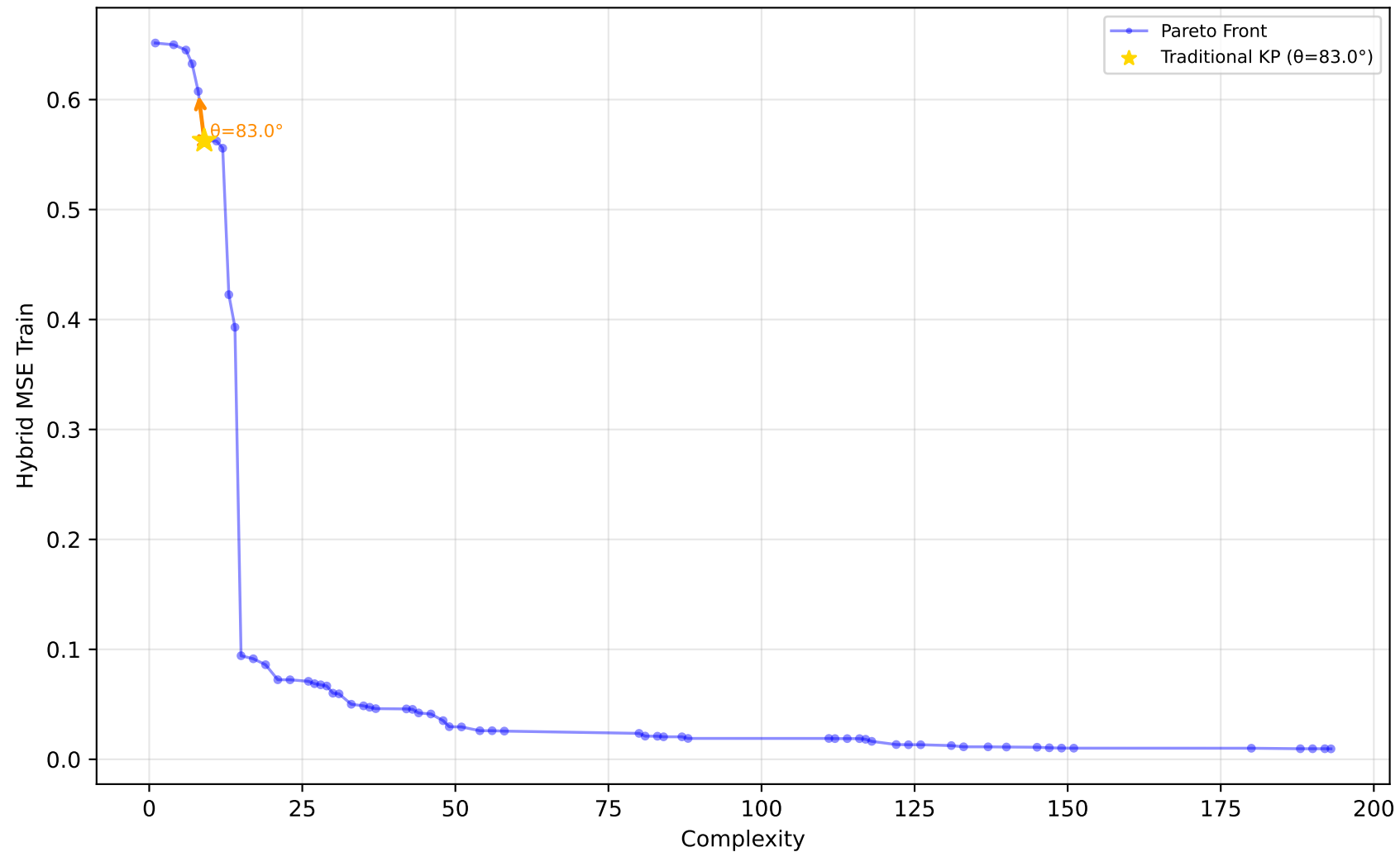
556_analcatdata_apnea2 - Run 19 - MVP - Hybrid MSE Train \lambda_1=0.00, \lambda_2=0.00, \lambda_3=0.00 | Difficulty: 1.00 | Method: hmr
