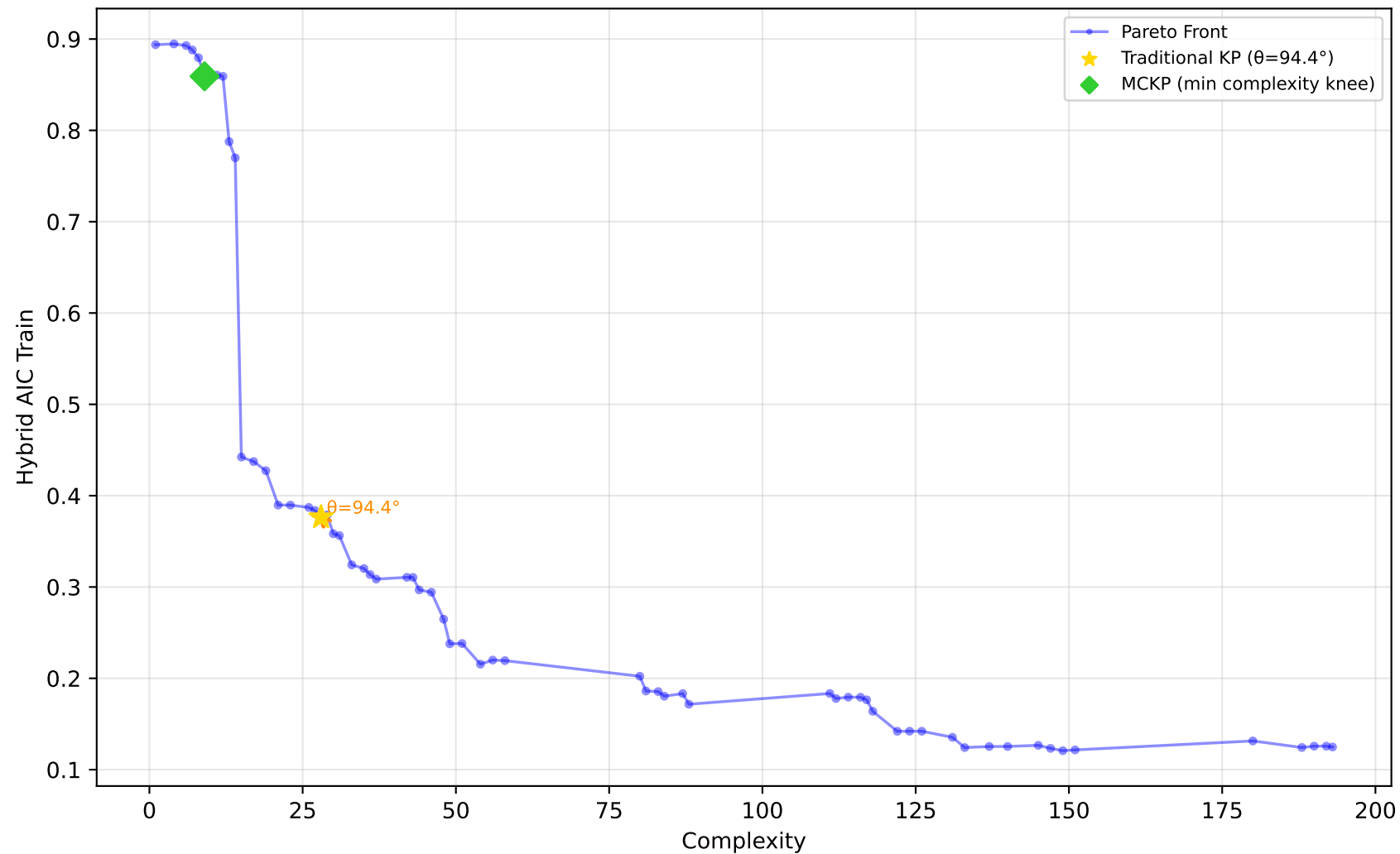
556_analcatdata_apnea2 - Run 19 - SVP - Hybrid AIC Train \lambda_1=0.00, \lambda_2=0.00, \lambda_3=0.00 | Difficulty: 1.00 | Method: hmr
