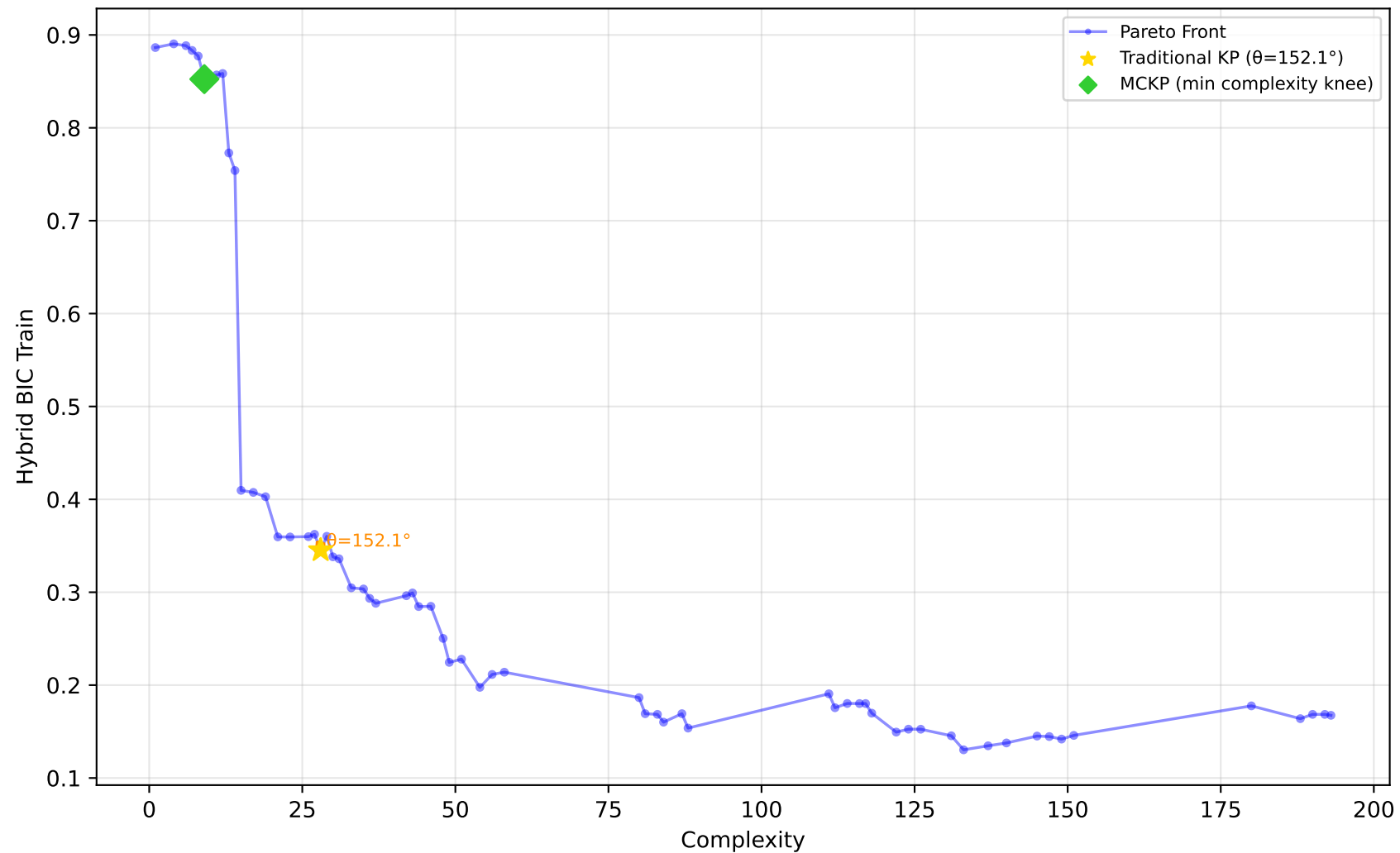
556_analcatdata_apnea2 - Run 19 - SVP - Hybrid BIC Train \lambda_1=0.00, \lambda_2=0.00, \lambda_3=0.00 | Difficulty: 1.00 | Method: hmr
