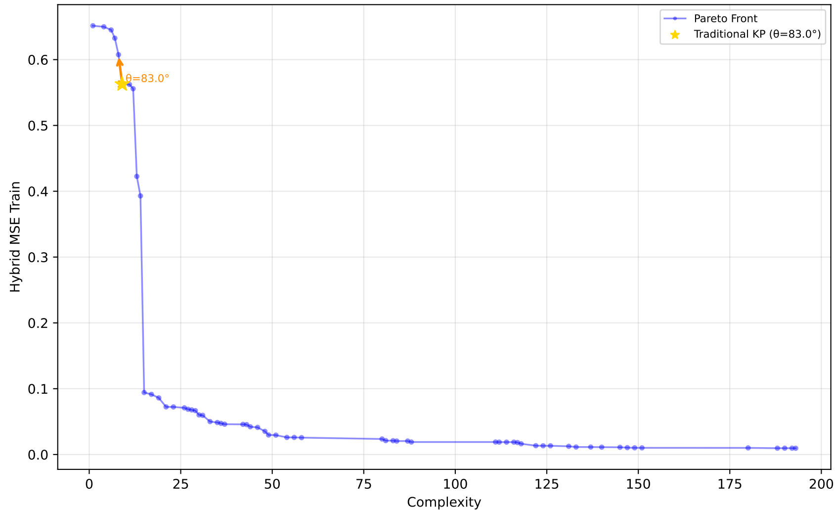
556_analcatdata_apnea2 - Run 19 - SVP - Hybrid MSE Train \lambda_1=0.00, \lambda_2=0.00, \lambda_3=0.00 | Difficulty: 1.00 | Method: hmr
