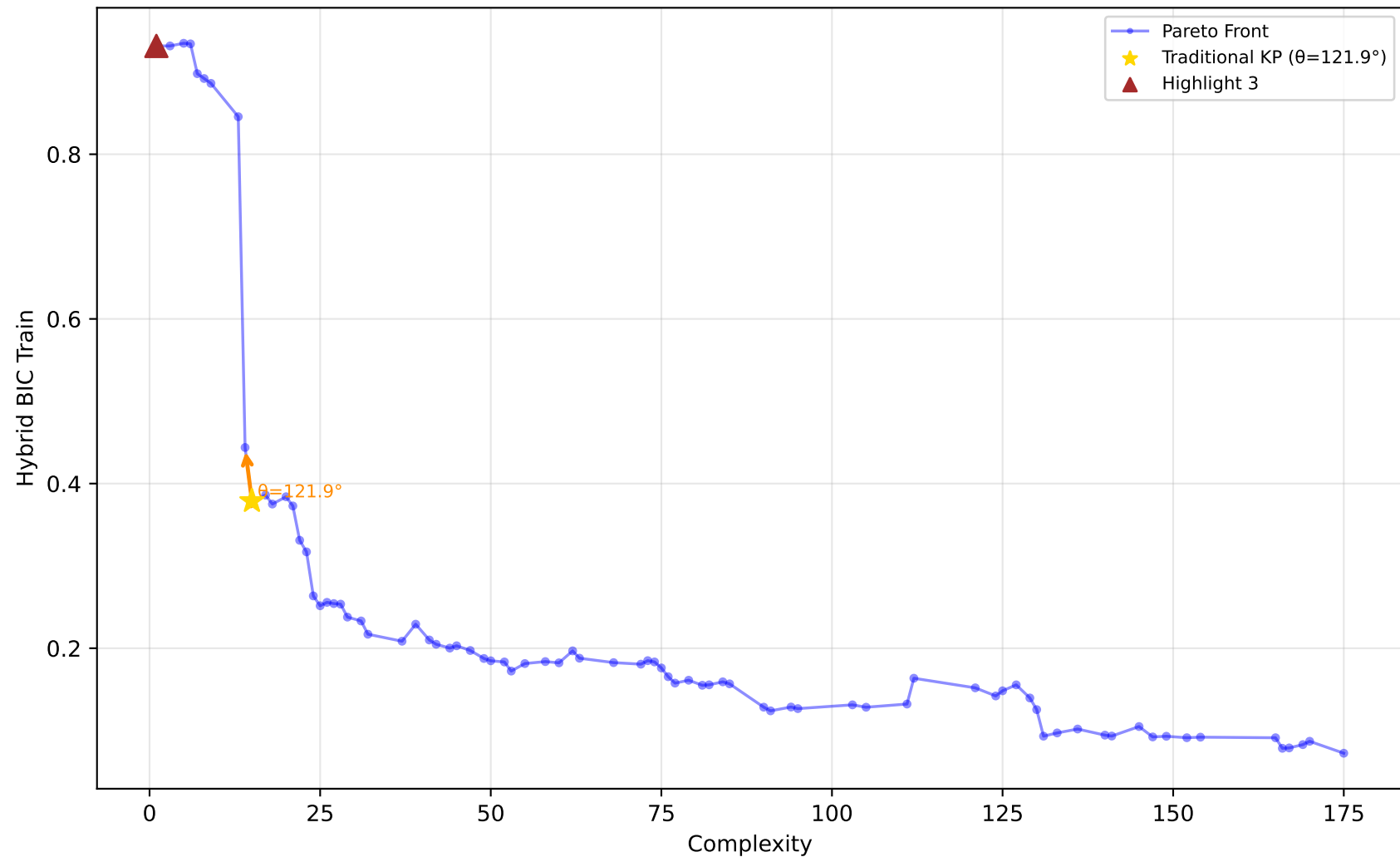
556_analcatdata_apnea2 - Run 1 - MVP - Hybrid BIC Train \lambda_1=0.00, \lambda_2=0.00, \lambda_3=0.00 | Difficulty: 1.00 | Method: hmr
