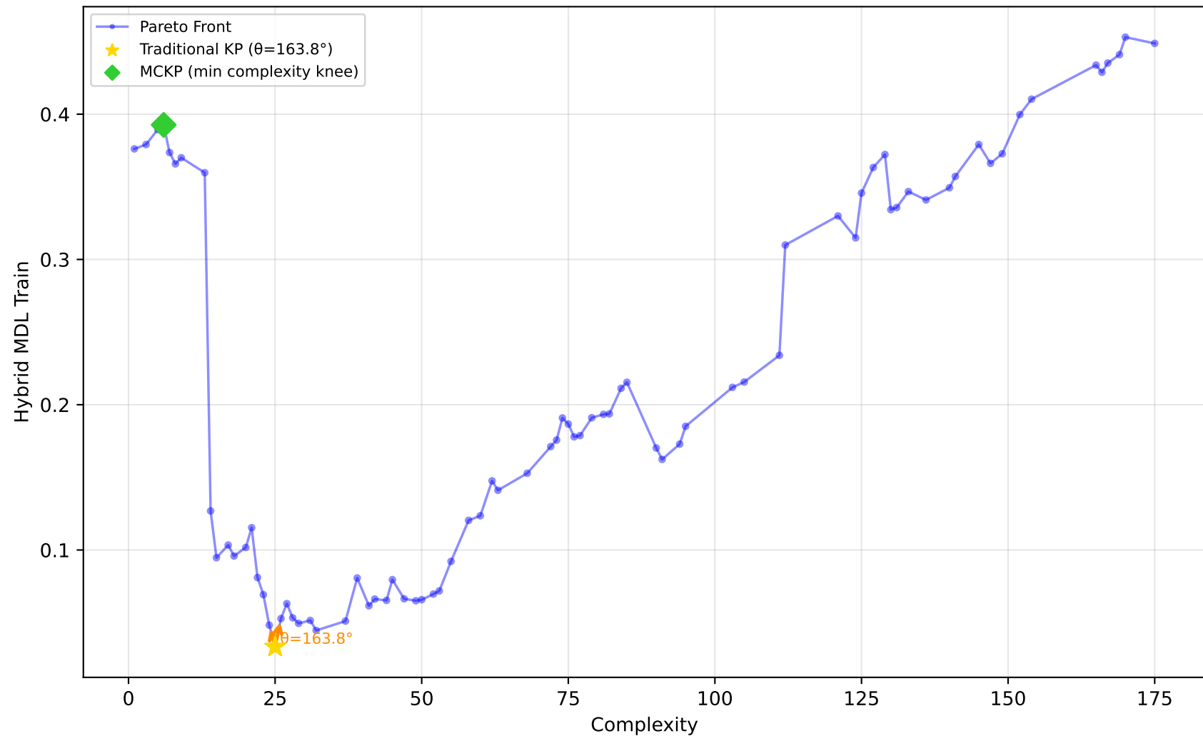
556_analcatdata_apnea2 - Run 1 - SVP - Hybrid MDL Train \lambda_1=0.00, \lambda_2=0.00, \lambda_3=0.00 | Difficulty: 1.00 | Method: hmr
