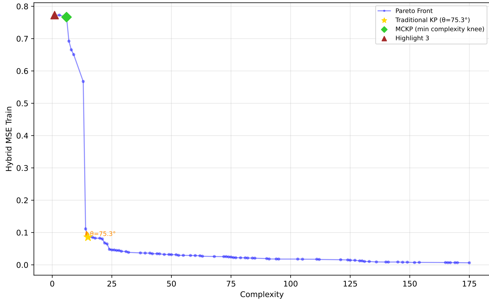
556_analcatdata_apnea2 - Run 1 - SVP - Hybrid MSE Train \lambda_1=0.00, \lambda_2=0.00, \lambda_3=0.00 | Difficulty: 1.00 | Method: hmr
