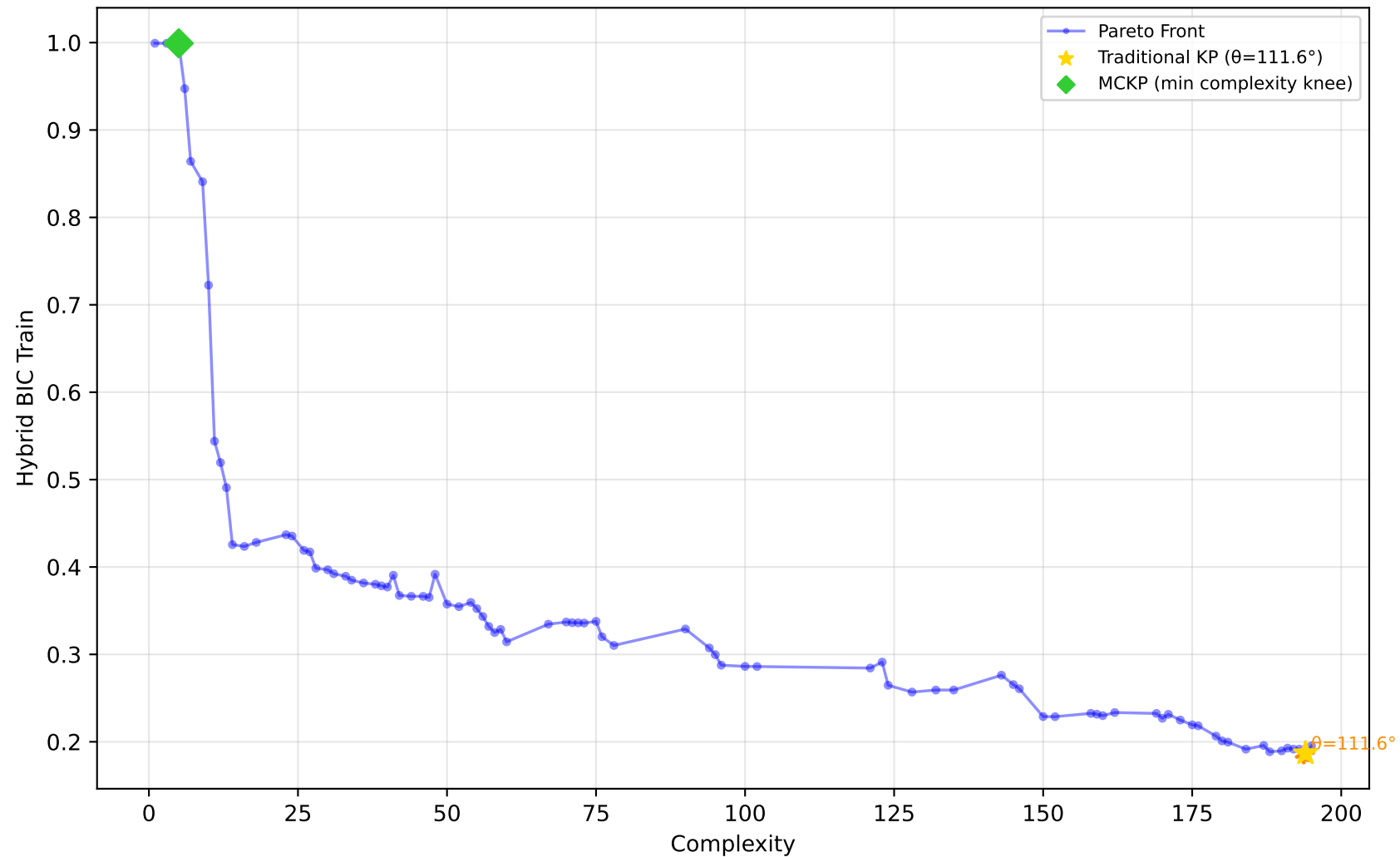
556_analcatdata_apnea2 - Run 20 - MVP - Hybrid BIC Train \lambda_1=0.00, \lambda_2=0.00, \lambda_3=0.00 | Difficulty: 1.00 | Method: hmr
