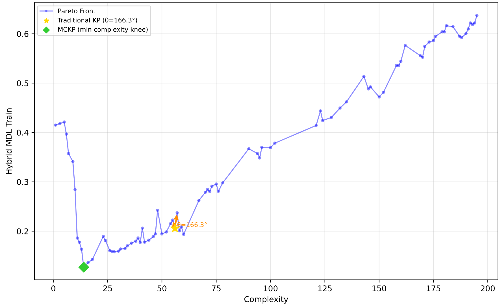
556_analcatdata_apnea2 - Run 20 - MVP - Hybrid MDL Train \lambda_1=0.00, \lambda_2=0.00, \lambda_3=0.00 | Difficulty: 1.00 | Method: hmr
