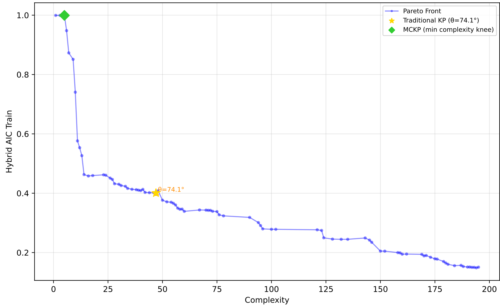
556_analcatdata_apnea2 - Run 20 - SVP - Hybrid AIC Train \lambda_1=0.00, \lambda_2=0.00, \lambda_3=0.00 | Difficulty: 1.00 | Method: hmr
