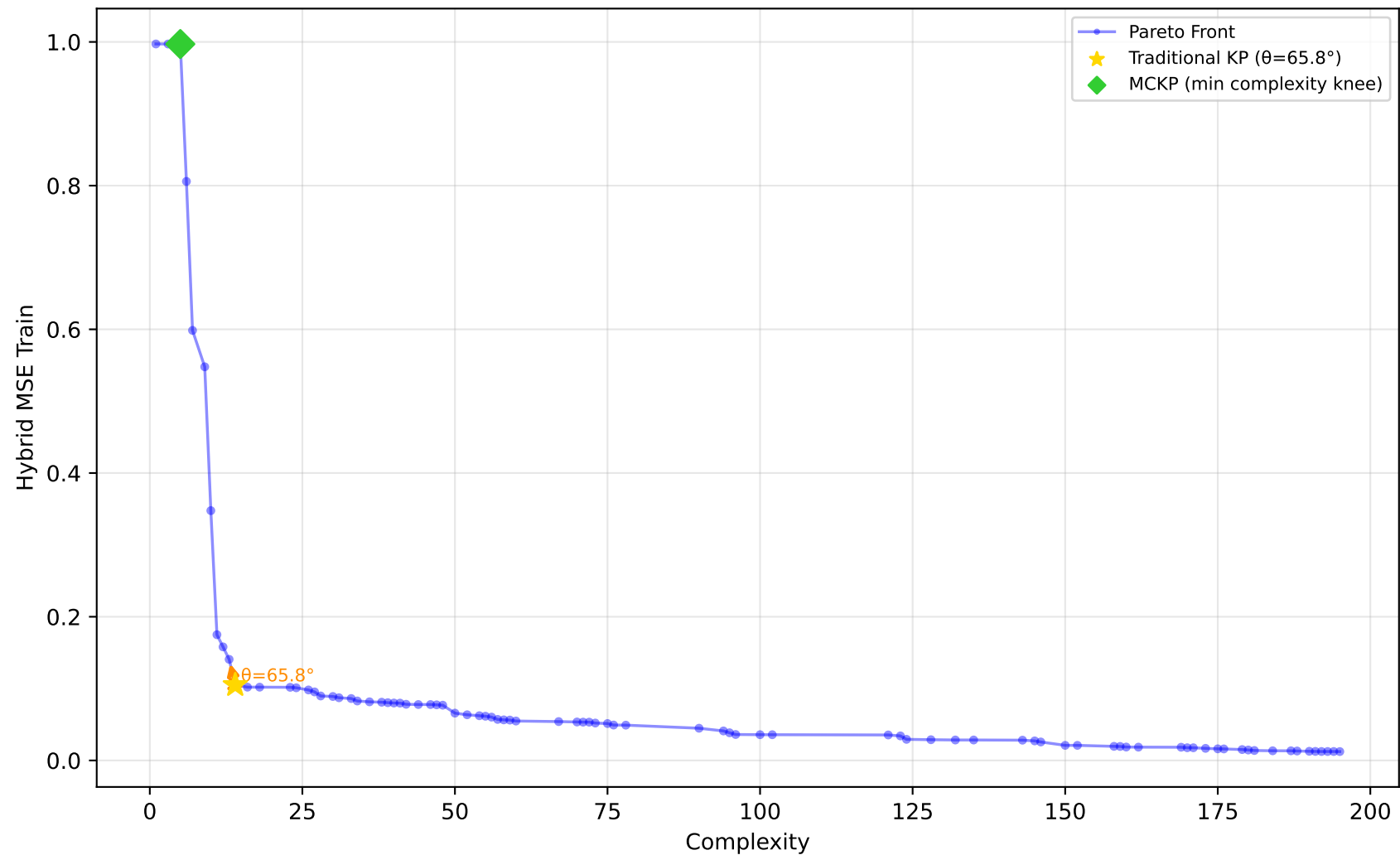
556_analcatdata_apnea2 - Run 20 - SVP - Hybrid MSE Train \lambda_1=0.00, \lambda_2=0.00, \lambda_3=0.00 | Difficulty: 1.00 | Method: hmr
