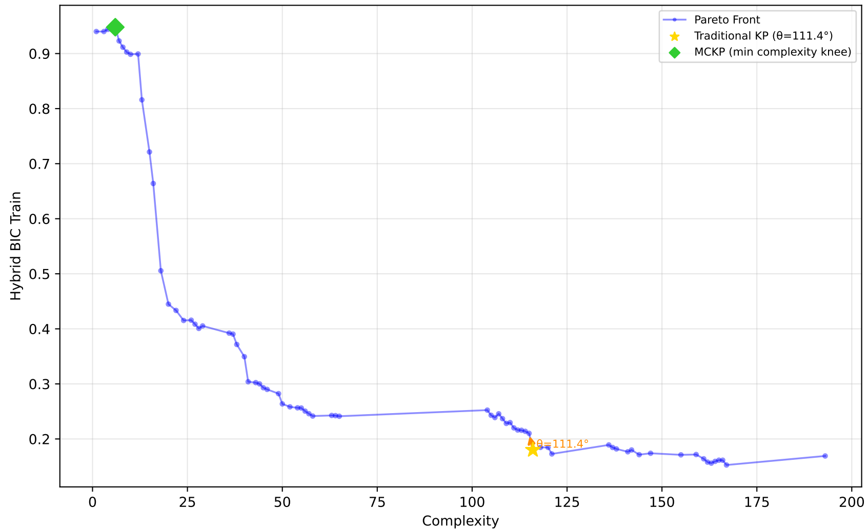
556_analcatdata_apnea2 - Run 21 - MVP - Hybrid BIC Train \lambda_1=0.00, \lambda_2=0.00, \lambda_3=0.00 | Difficulty: 1.00 | Method: hmr
