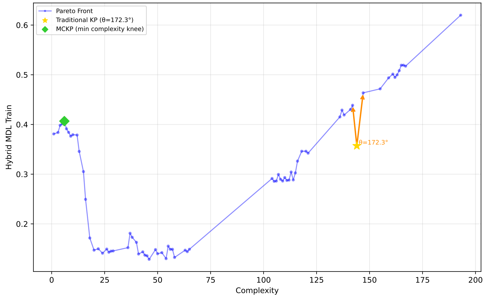
556_analcatdata_apnea2 - Run 21 - MVP - Hybrid MDL Train \lambda_1=0.00, \lambda_2=0.00, \lambda_3=0.00 | Difficulty: 1.00 | Method: hmr
