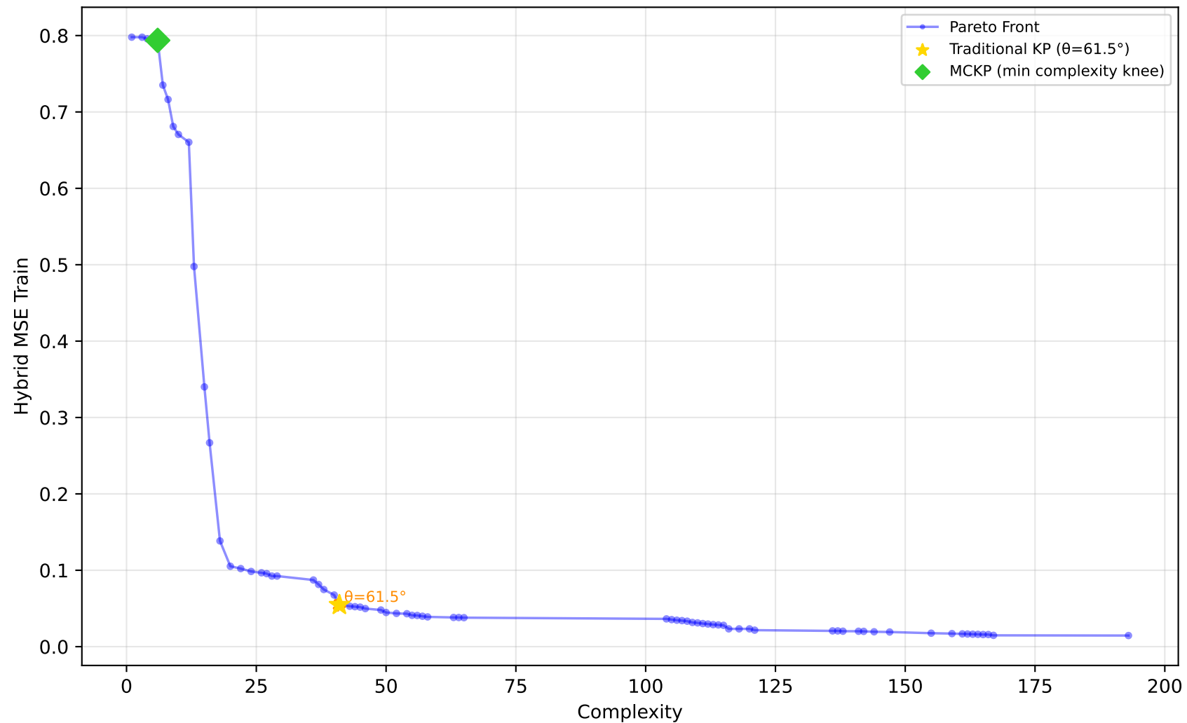
556_analcatdata_apnea2 - Run 21 - MVP - Hybrid MSE Train \lambda_1=0.00, \lambda_2=0.00, \lambda_3=0.00 | Difficulty: 1.00 | Method: hmr
