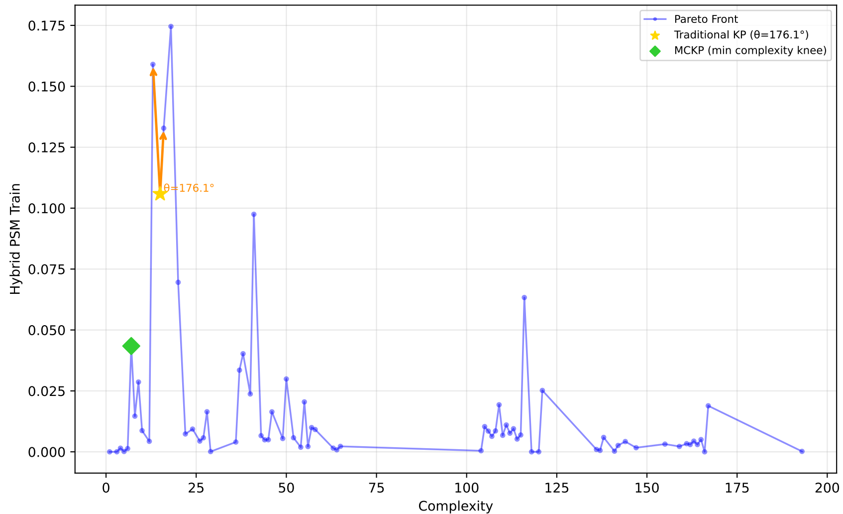
556_analcatdata_apnea2 - Run 21 - SVP - Hybrid PSM Train \lambda_1=0.00, \lambda_2=0.00, \lambda_3=0.00 | Difficulty: 1.00 | Method: hmr
