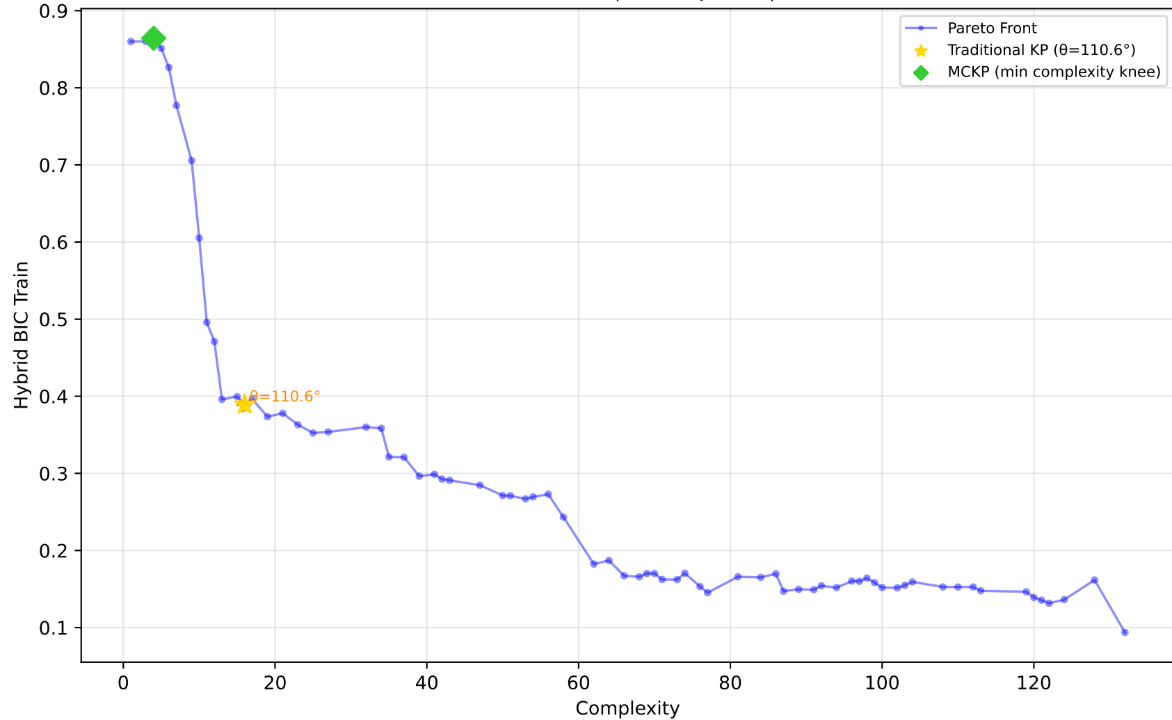
556_analcatdata_apnea2 - Run 22 - MVP - Hybrid BIC Train \lambda_1=0.00, \lambda_2=0.00, \lambda_3=0.00 | Difficulty: 0.93 | Method: hmr
