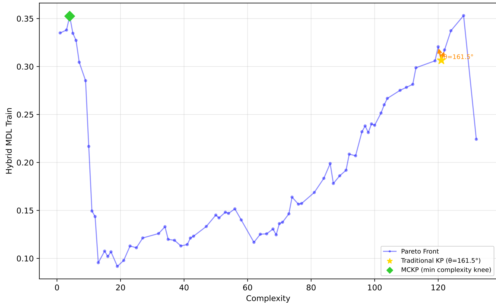
556_analcatdata_apnea2 - Run 22 - MVP - Hybrid MDL Train \lambda_1=0.00, \lambda_2=0.00, \lambda_3=0.00 | Difficulty: 0.93 | Method: hmr
