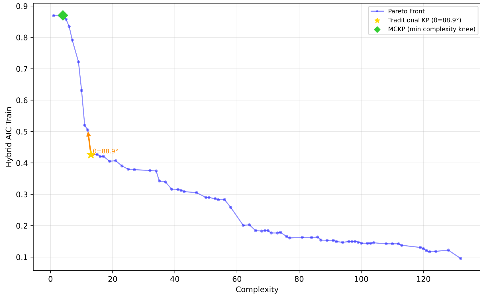
556_analcatdata_apnea2 - Run 22 - SVP - Hybrid AIC Train \lambda_1=0.00, \lambda_2=0.00, \lambda_3=0.00 | Difficulty: 0.93 | Method: hmr
