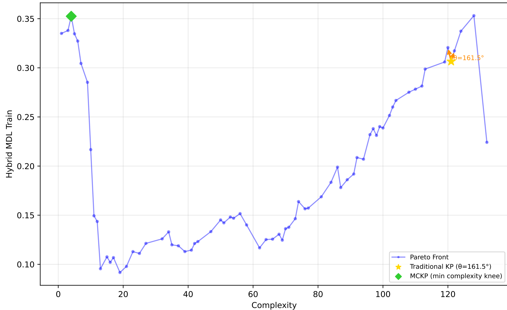
556_analcatdata_apnea2 - Run 22 - SVP - Hybrid MDL Train \lambda_1=0.00, \lambda_2=0.00, \lambda_3=0.00 | Difficulty: 0.93 | Method: hmr
