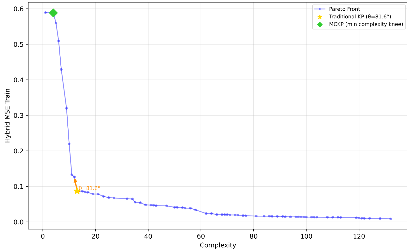
556_analcatdata_apnea2 - Run 22 - SVP - Hybrid MSE Train \lambda_1=0.00, \lambda_2=0.00, \lambda_3=0.00 | Difficulty: 0.93 | Method: hmr
