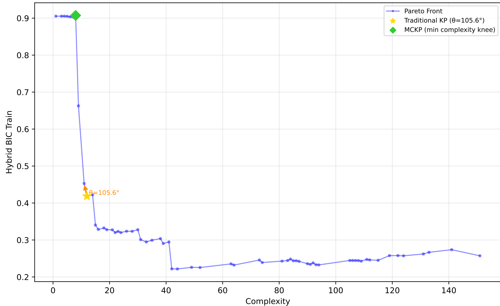
556_analcatdata_apnea2 - Run 23 - MVP - Hybrid BIC Train \lambda_1=0.00, \lambda_2=0.00, \lambda_3=0.00 | Difficulty: 1.00 | Method: hmr
