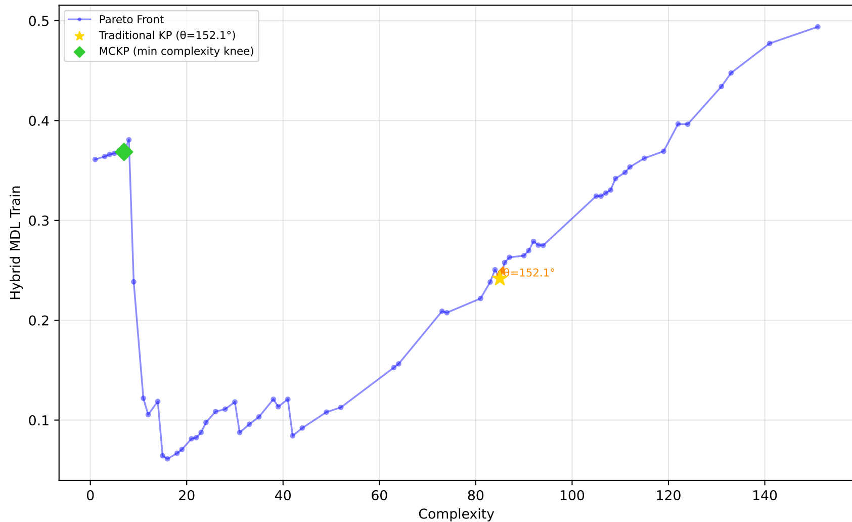
556_analcatdata_apnea2 - Run 23 - MVP - Hybrid MDL Train \lambda_1=0.00, \lambda_2=0.00, \lambda_3=0.00 | Difficulty: 1.00 | Method: hmr
