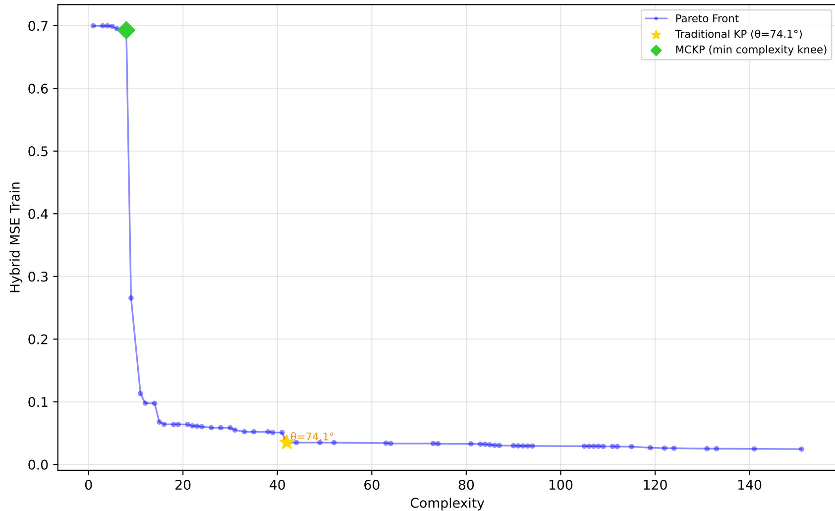
556_analcatdata_apnea2 - Run 23 - SVP - Hybrid MSE Train \lambda_1=0.00, \lambda_2=0.00, \lambda_3=0.00 | Difficulty: 1.00 | Method: hmr
