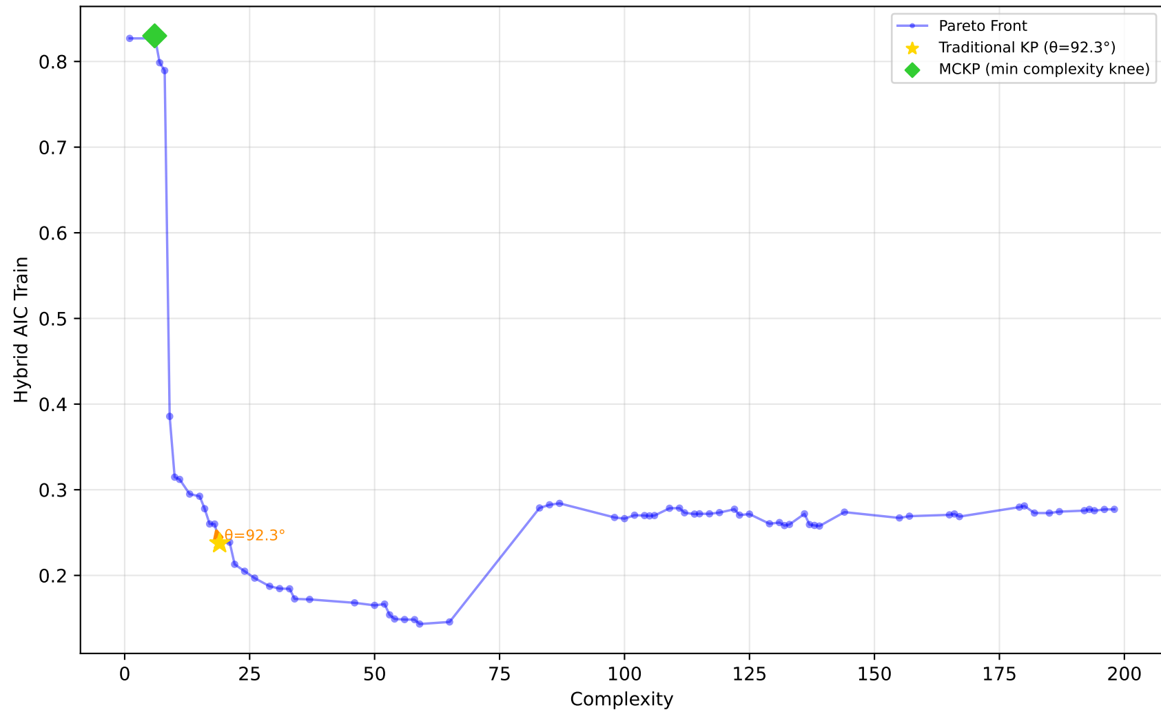
556_analcatdata_apnea2 - Run 24 - MVP - Hybrid AIC Train \lambda_1=0.00 , \lambda_2=0.00 , \lambda_3=0.00 | Difficulty: 1.00 | Method: hmr
