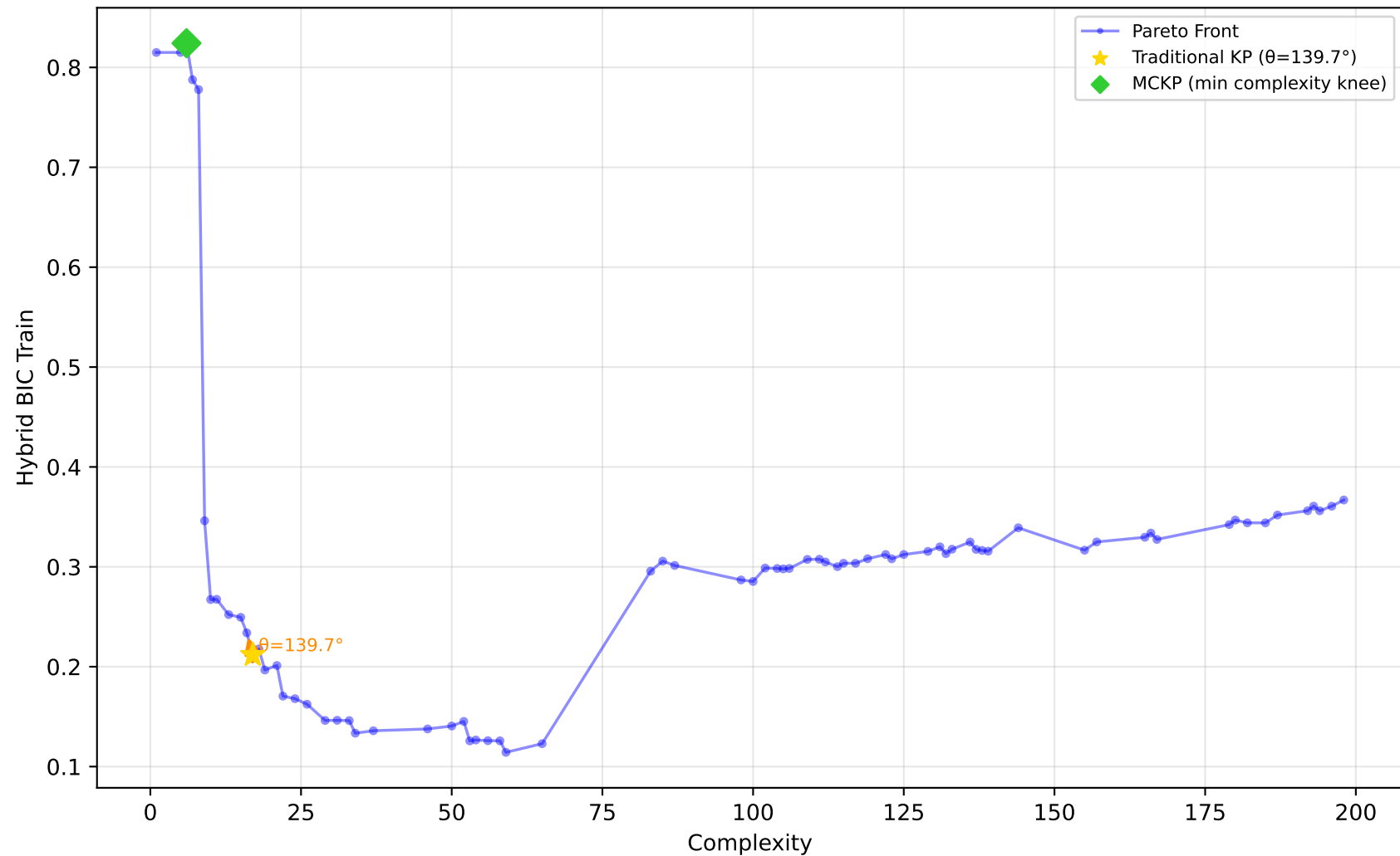
556_analcatdata_apnea2 - Run 24 - MVP - Hybrid BIC Train \lambda_1=0.00, \lambda_2=0.00, \lambda_3=0.00 | Difficulty: 1.00 | Method: hmr
