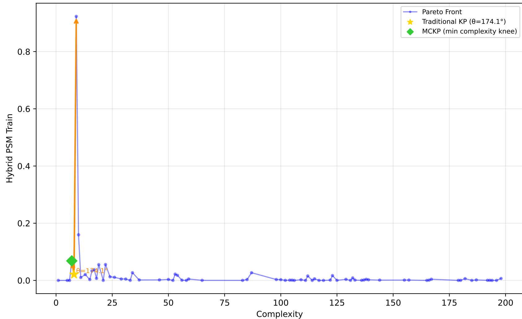
556_analcatdata_apnea2 - Run 24 - MVP - Hybrid PSM Train \lambda_1=0.00, \lambda_2=0.00, \lambda_3=0.00 | Difficulty: 1.00 | Method: hmr
