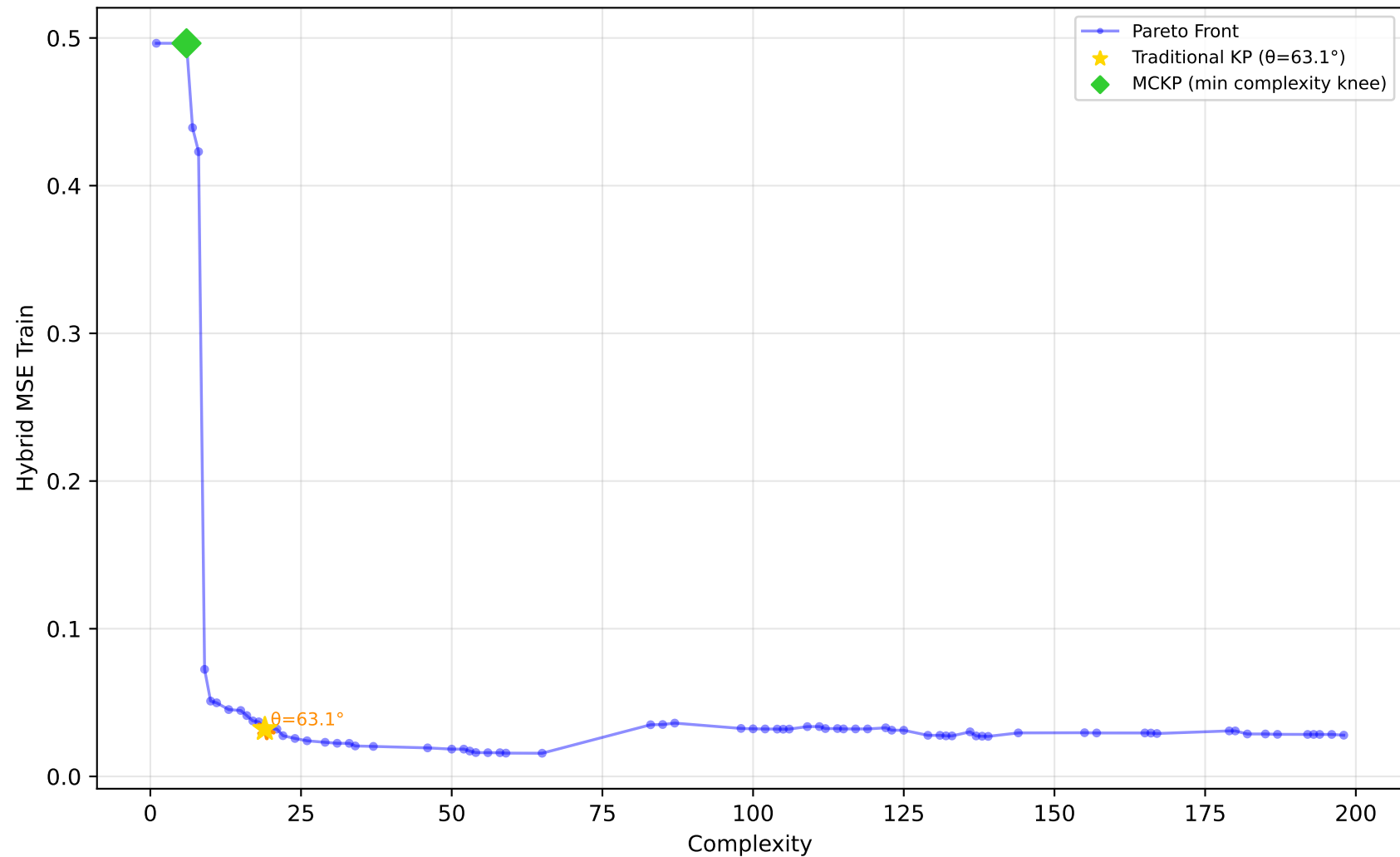
556_analcatdata_apnea2 - Run 24 - SVP - Hybrid MSE Train \lambda_1=0.00, \lambda_2=0.00, \lambda_3=0.00 | Difficulty: 1.00 | Method: hmr
