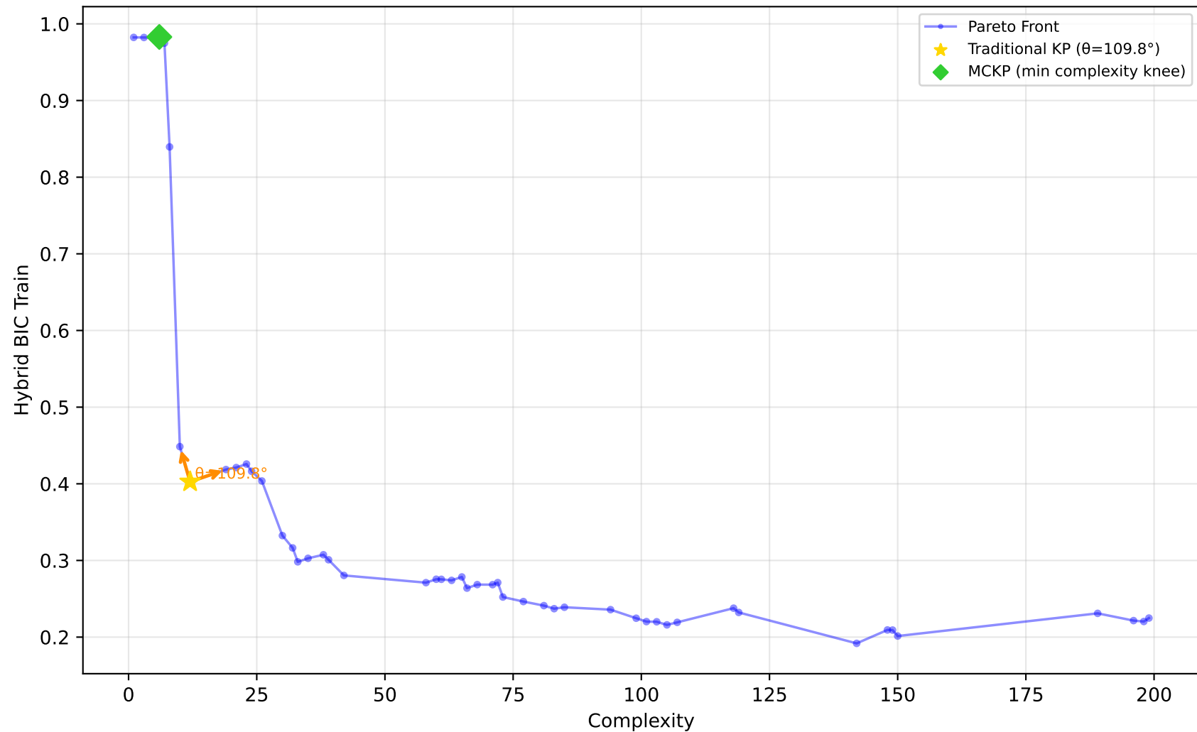
556_analcatdata_apnea2 - Run 25 - MVP - Hybrid BIC Train \lambda_1=0.00, \lambda_2=0.00, \lambda_3=0.00 | Difficulty: 1.00 | Method: hmr
