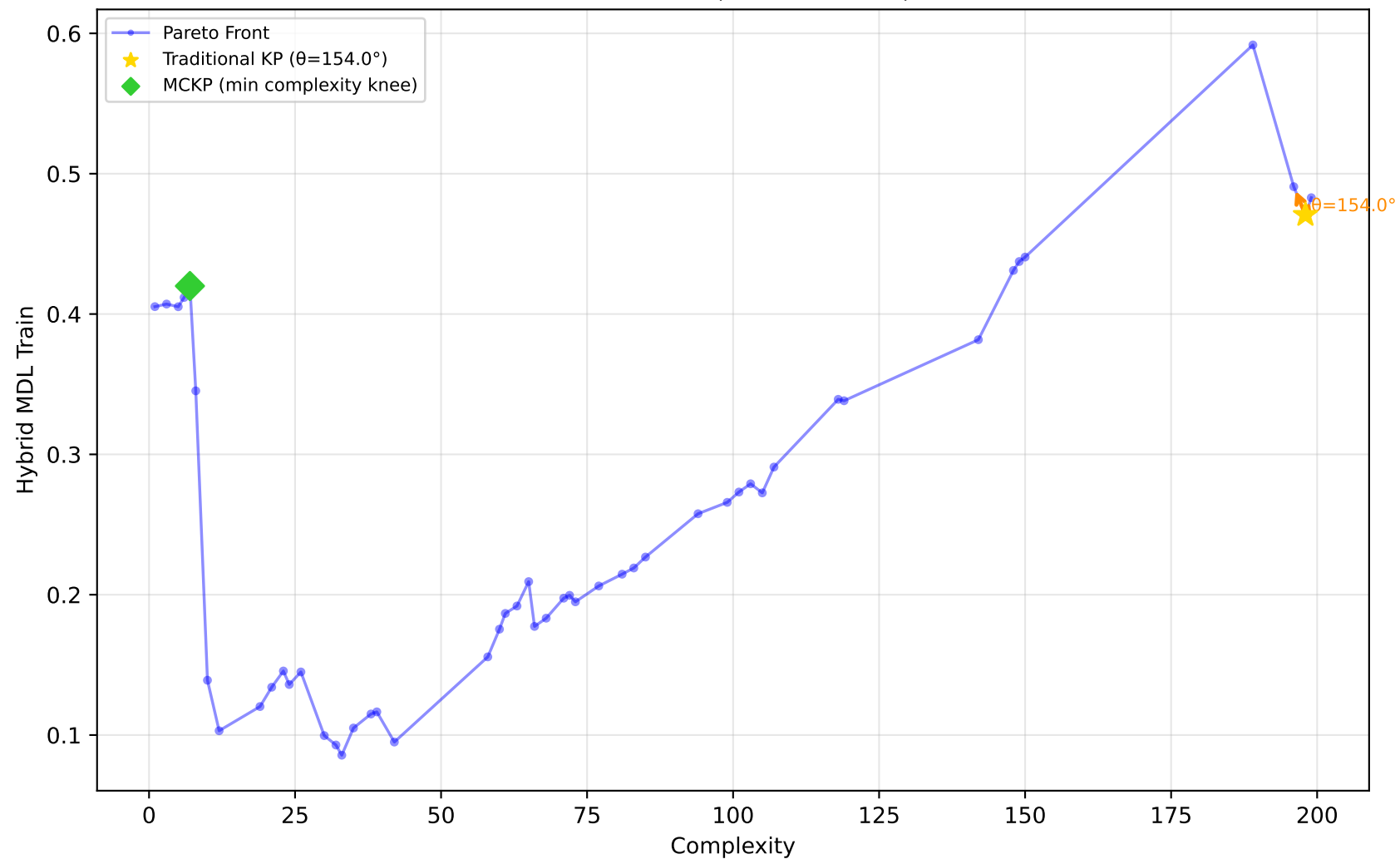
556_analcatdata_apnea2 - Run 25 - MVP - Hybrid MDL Train \lambda_1=0.00, \lambda_2=0.00, \lambda_3=0.00 | Difficulty: 1.00 | Method: hmr
