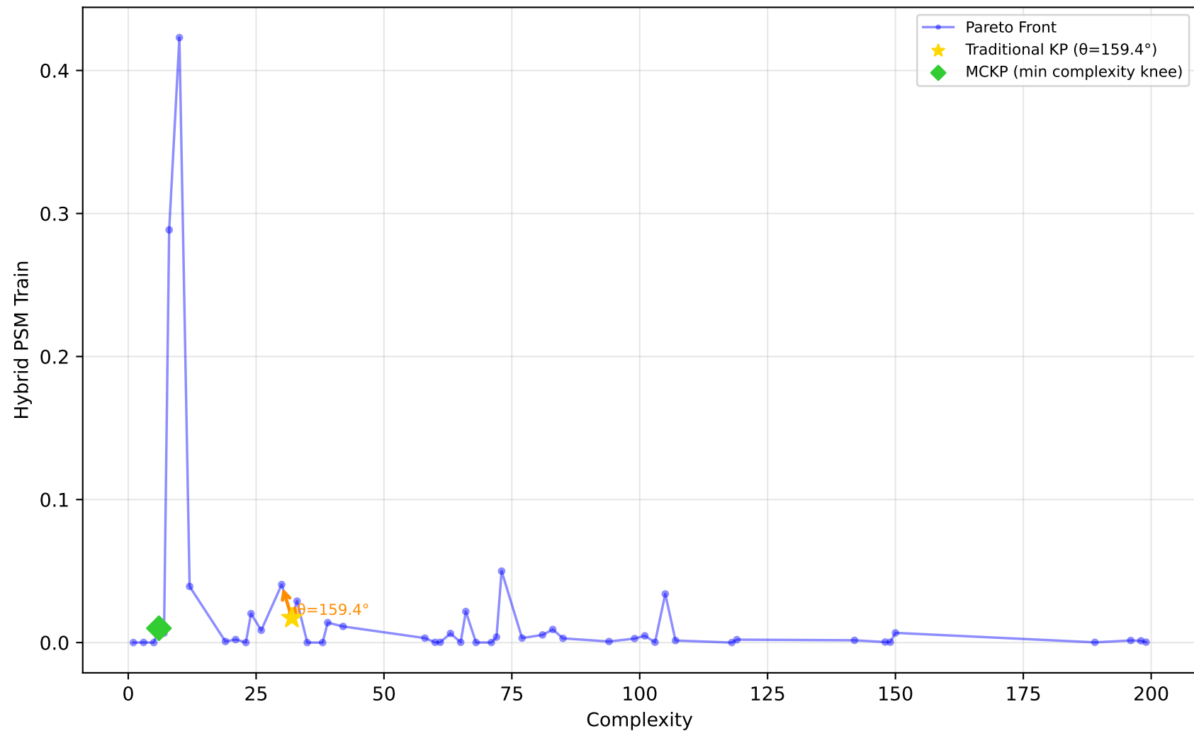
556_analcatdata_apnea2 - Run 25 - MVP - Hybrid PSM Train \lambda_1=0.00, \lambda_2=0.00, \lambda_3=0.00 | Difficulty: 1.00 | Method: hmr
