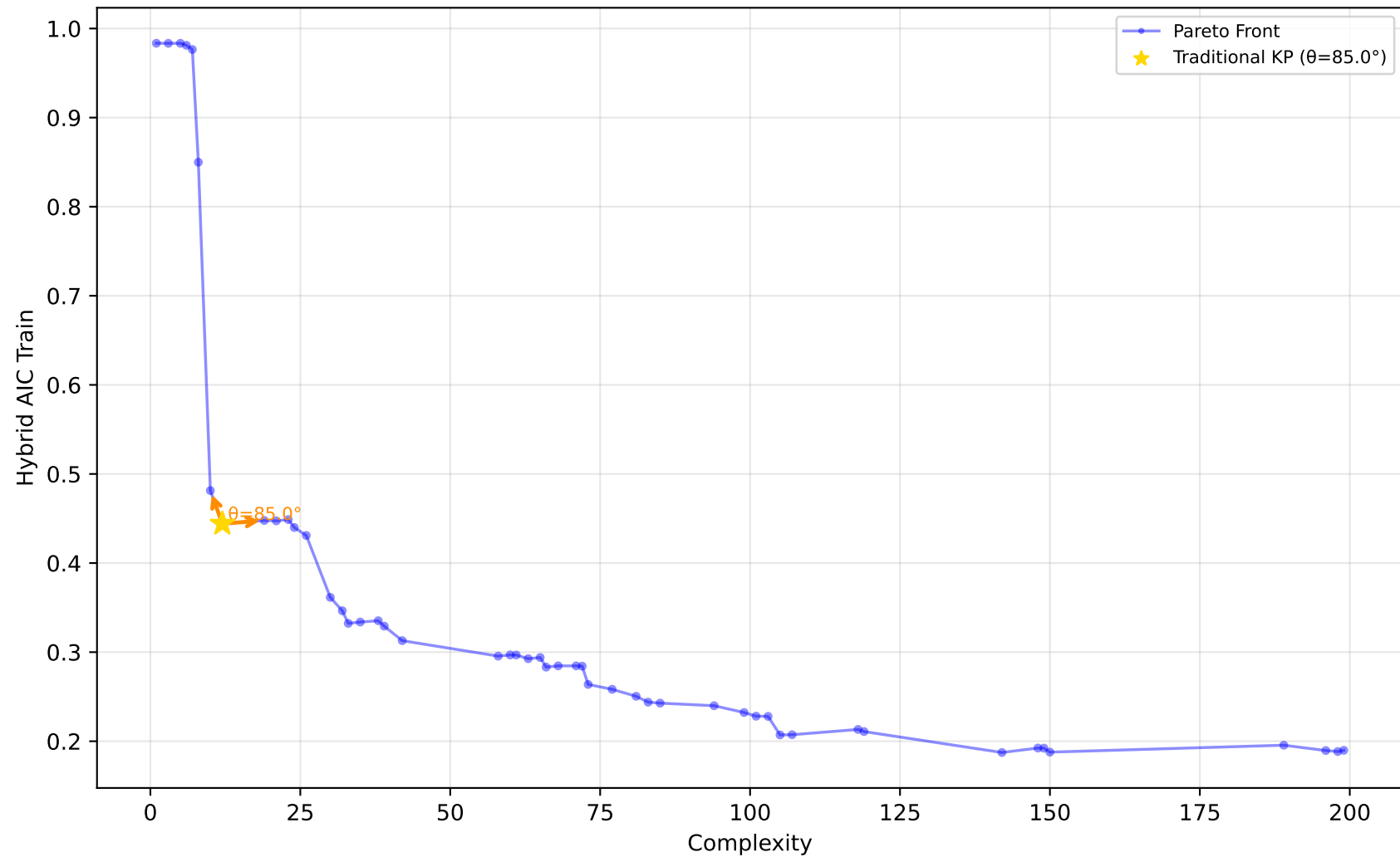
556_analcatdata_apnea2 - Run 25 - SVP - Hybrid AIC Train \lambda_1=0.00, \lambda_2=0.00, \lambda_3=0.00 | Difficulty: 1.00 | Method: hmr
