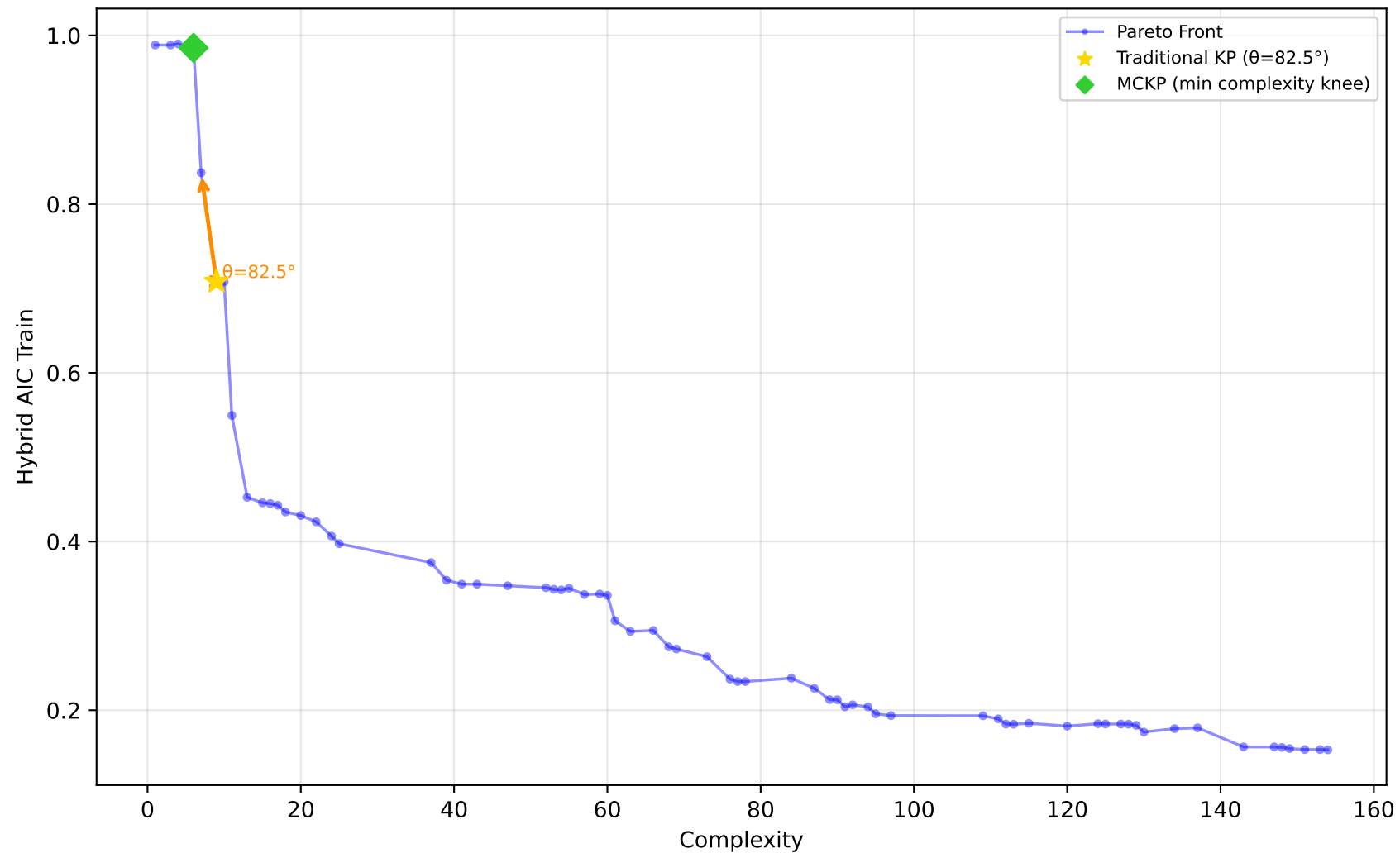
556_analcatdata_apnea2 - Run 26 - MVP - Hybrid AIC Train \lambda_1=0.00 , \lambda_2=0.00 , \lambda_3=0.00 | Difficulty: 1.00 | Method: hmr
